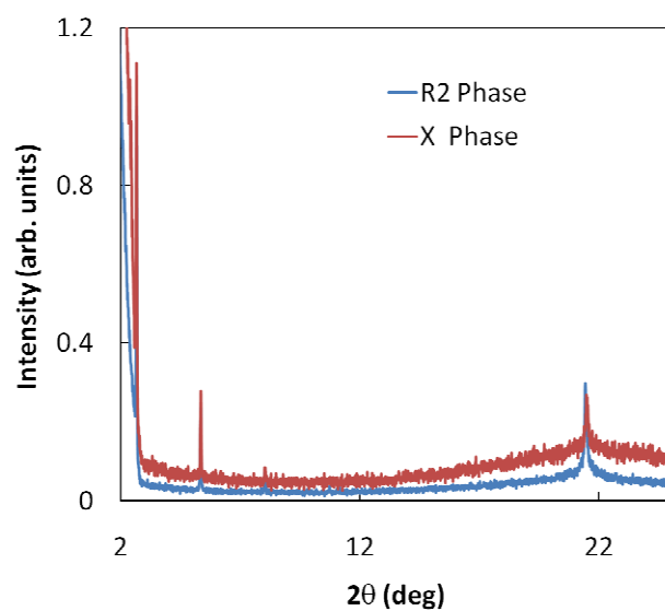
Figure SI-1: X-ray diffraction profiles in the R2 and X phases for \rho = 0.06 composites. The pattern is essentially identical in the two phases.
