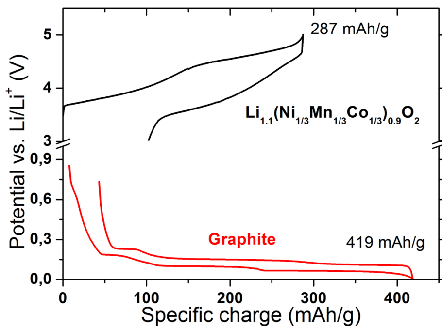
Figure A: First electrochemical cycle of \text{Li}_{1.1}(\text{Ni}_{1/3}\text{Mn}_{1/3}\text{Co}_{1/3})_{0.9}\text{O}_2 and graphite electrodes in a coin-like cell for comparison with the electrochemistry of these active materials in the in situ neutron powder diffraction (NPD) cell.
