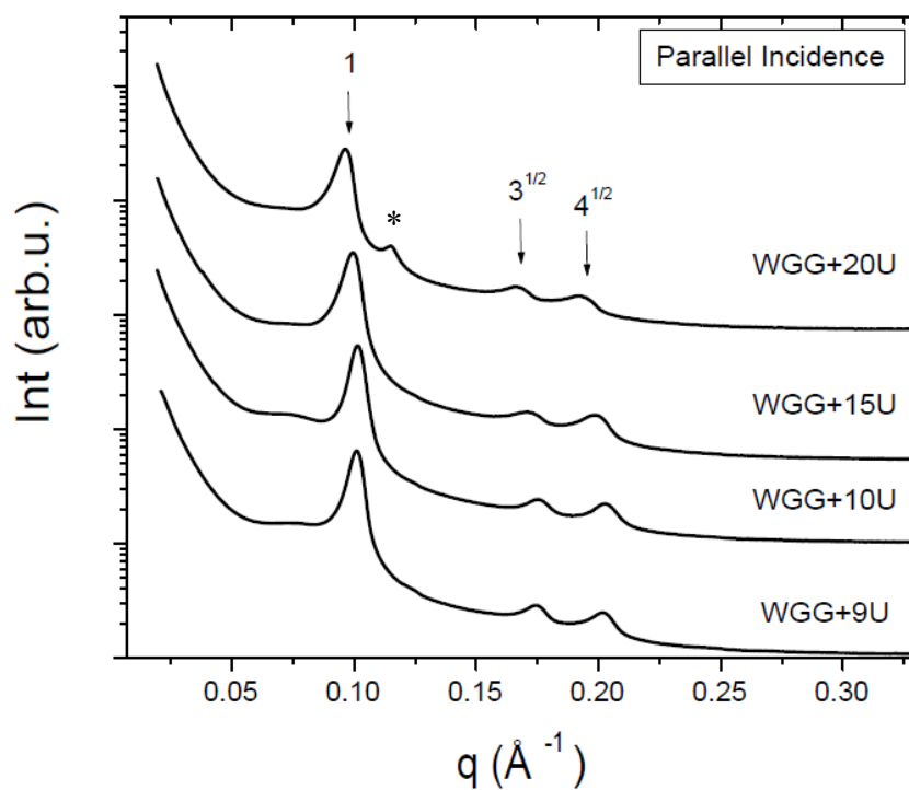
Fig. S1. SAXS curves of WGG+9U, WGG+10U, WGG+15U and WGG+20U films with the X-ray beam parallel to the film plane.
