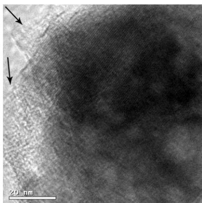
Figure S1. The TEM image of as-synthesized \text{Li}_2\text{FeSiO}_4/\text{C} .
