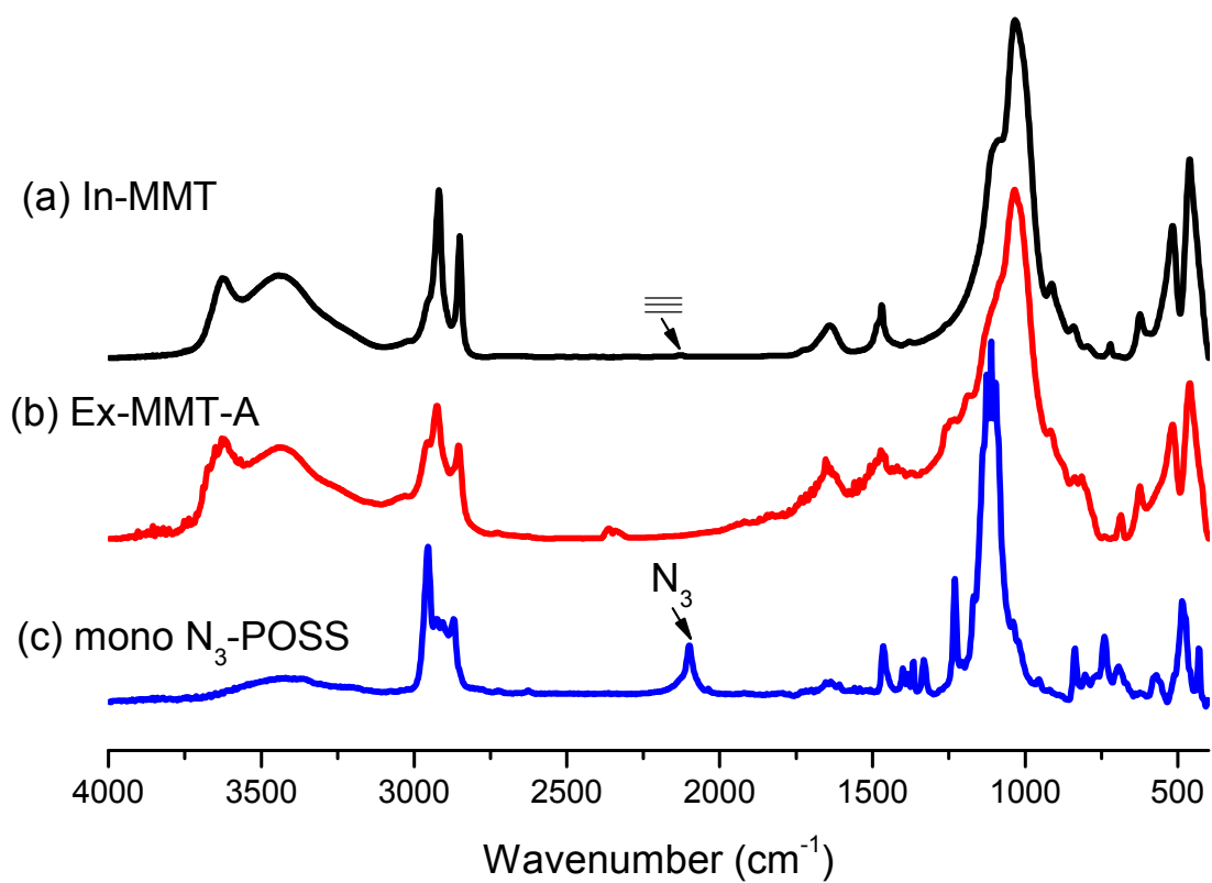
Figure S1: FTIR spectra of (a) In-MMT, (b) Ex-MMT-A, and (e) mono-N3-POSS
