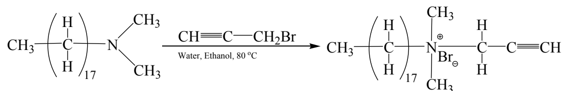
Scheme S1: The synthesis of PDS
