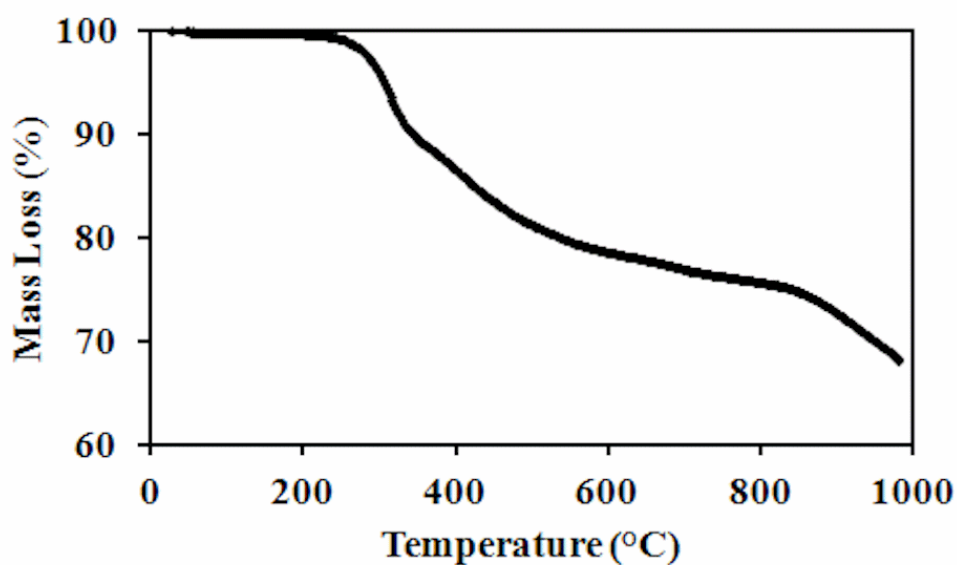
ESI Fig. 2 The TGA trace of the mass loss from of \text{Al}_2(\text{O}_3\text{PC}_6\text{H}_4\text{PO}_3)(\text{H}_2\text{O})_2\text{F}_2 \cdot 2\text{H}_2\text{O} .
