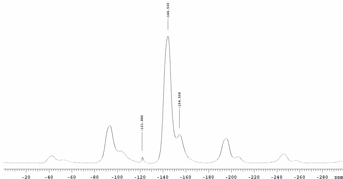
ESI Fig. 1 The ^{19}\text{F} MAS SS NMR spectrum of \text{Al}_2(\text{O}_3\text{PC}_6\text{H}_4\text{PO}_3)(\text{H}_2\text{O})_2\text{F}_2 \cdot 2\text{H}_2\text{O}
