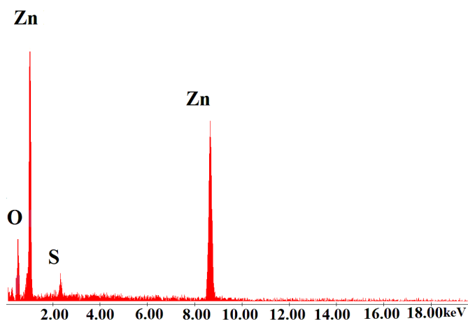
Fig. S2 The EDS spectrum on the annealed sample in Ar atmosphere showing a small amount of S Present.
