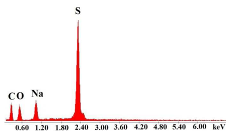
Fig. S1 EDS spectra of a) ZnO side b) PEDOT:PSS side of the polymer.
