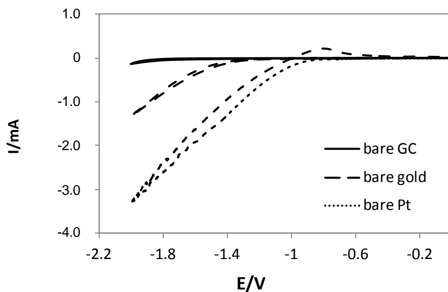
Figure S1. Cyclic voltammograms for platinum bare electrode (Pt - dotted curve), gold bare electrode (Au – dashed curve), and glassy carbon bare electrode (GC – black curve). Measurements were performed in PBS buffer solution, pH 7.
