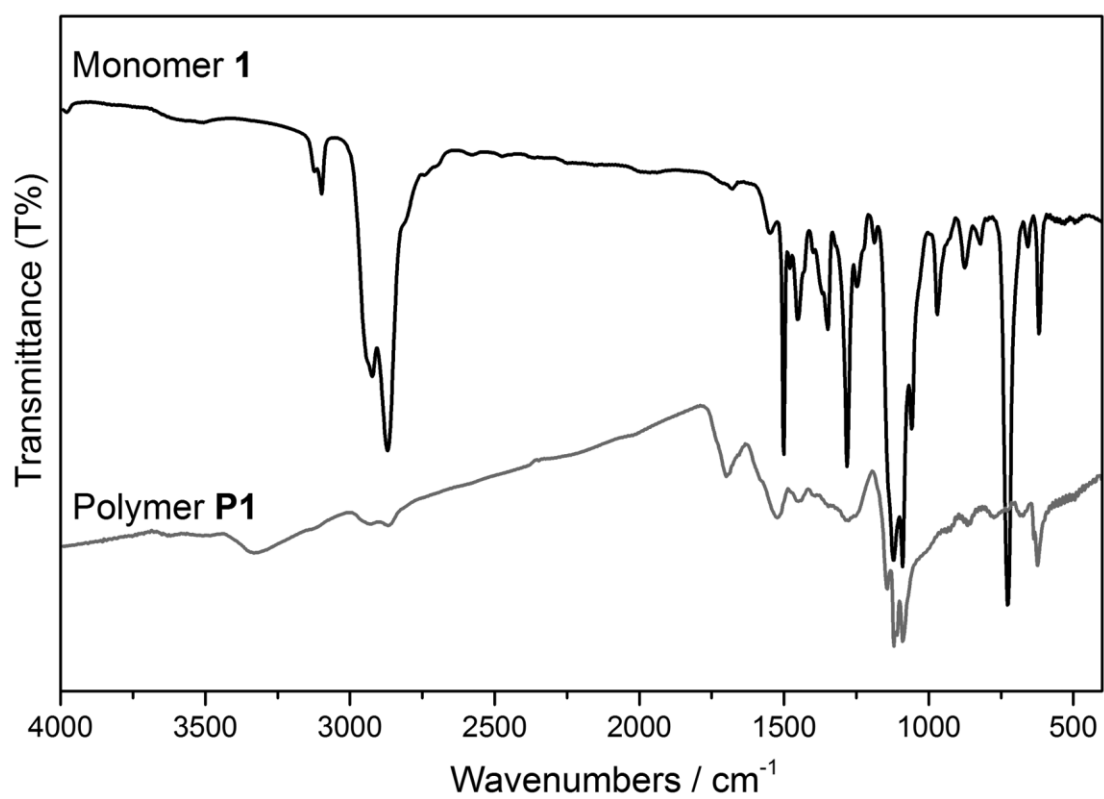
Supp. Info Figure 2: FTIR spectrum of Monomer 1 and P1
