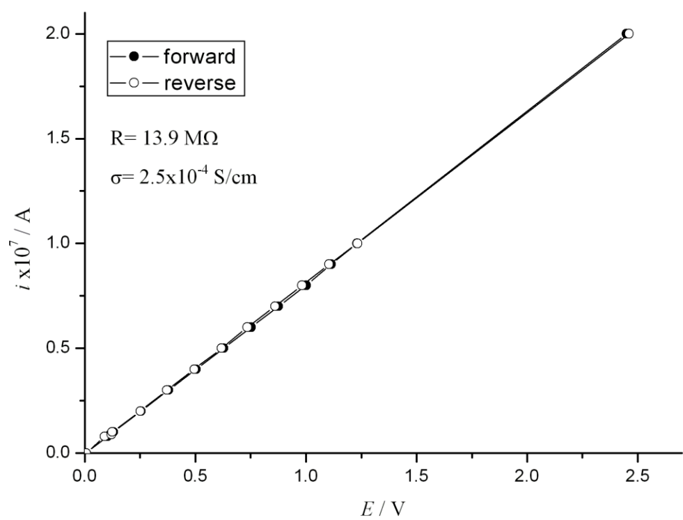
Supp. Info Figure 3: IVcurve of P1
