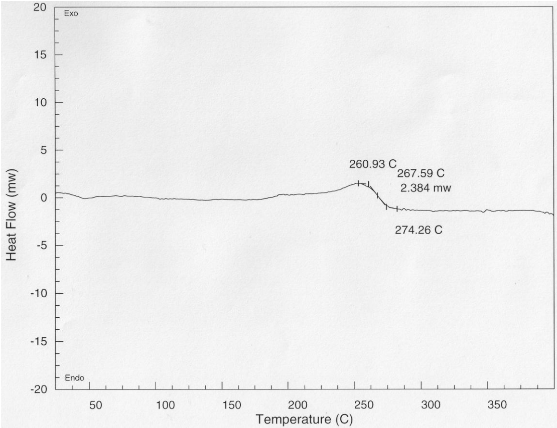
Supp Info Figure 1: DSC Thermogram of P1.
