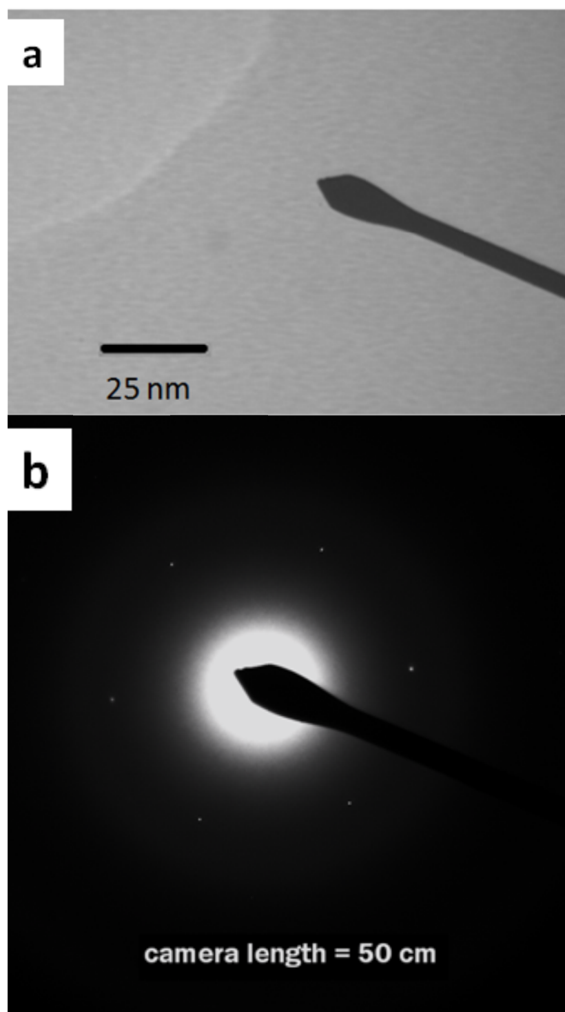
Figure S1. (a) A transmission electron micrograph (TEM) of exfoliated GUITAR and (b) the electron diffraction pattern. TEM's were conducted on a JEOL 1200 EX II TEM operated at 120 KV. The point charges are an indication of a crystal lattice structure. Amorphous carbon exhibits diffuse ring patterns.
