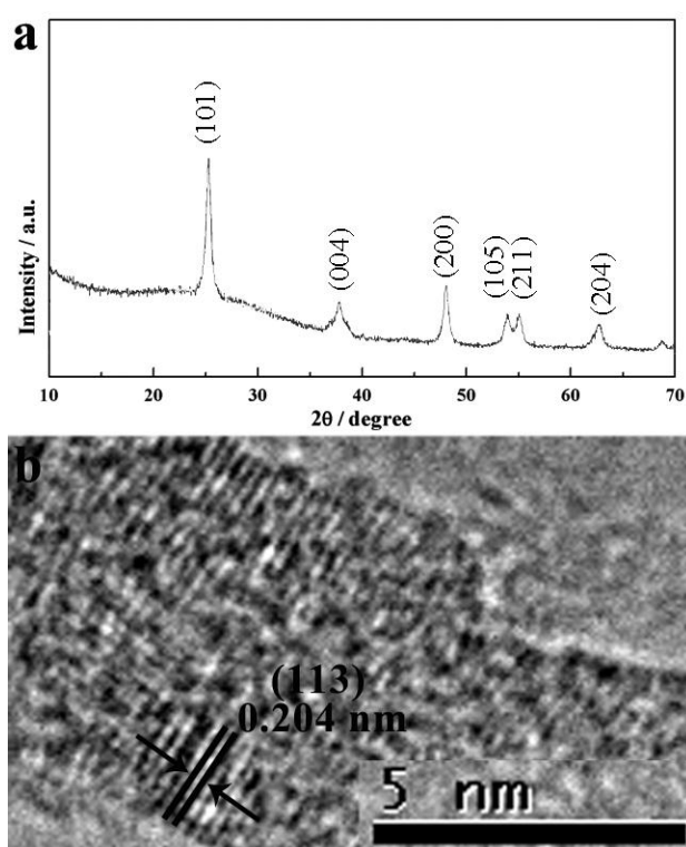
Fig. S1 XRD pattern and HRTEM image of the anatase TiO 2 nanotubes of 400 °C after charge/discharge cycles.
