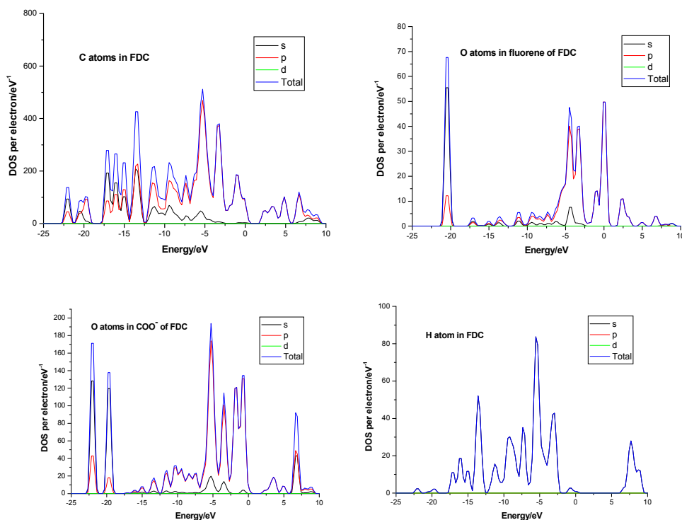
Figure S1. Total and partial electronic density of states (TDOS and PDOS) profiles for different atoms in pristine FDC.
