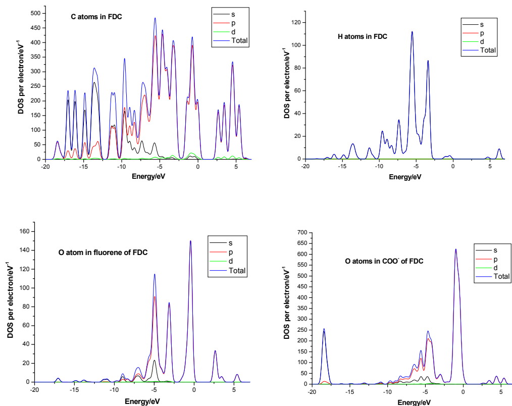
Figure S3. Total and partial electronic density of states (TDOS and PDOS) profiles for different atoms in FDC/ \text{Zn}_2\text{Al-LDH} system.
