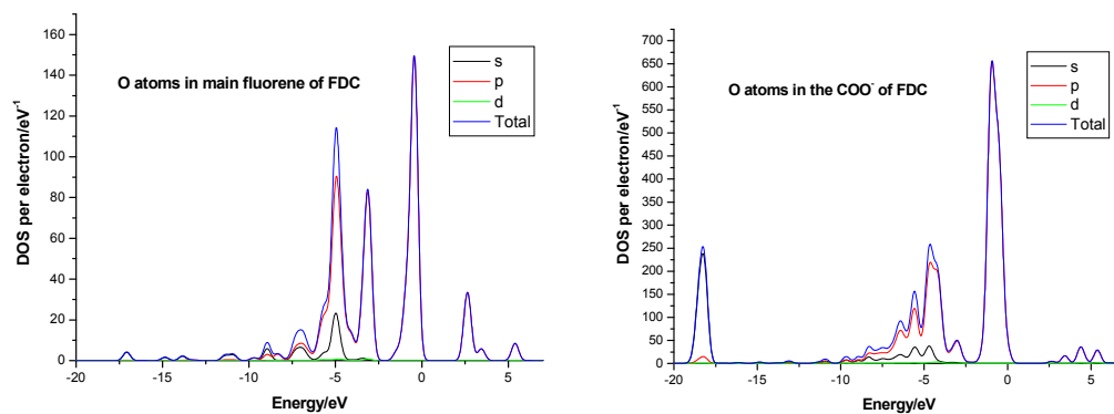
Figure S2. Total and partial electronic density of states (TDOS and PDOS) profiles for different atoms in FDC/Mg 2 Al-LDH system.
