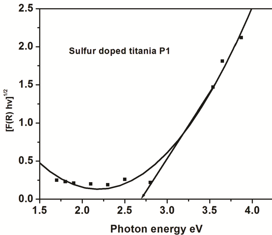
Figure S2. Tauc plots of S-doped titania P1.
