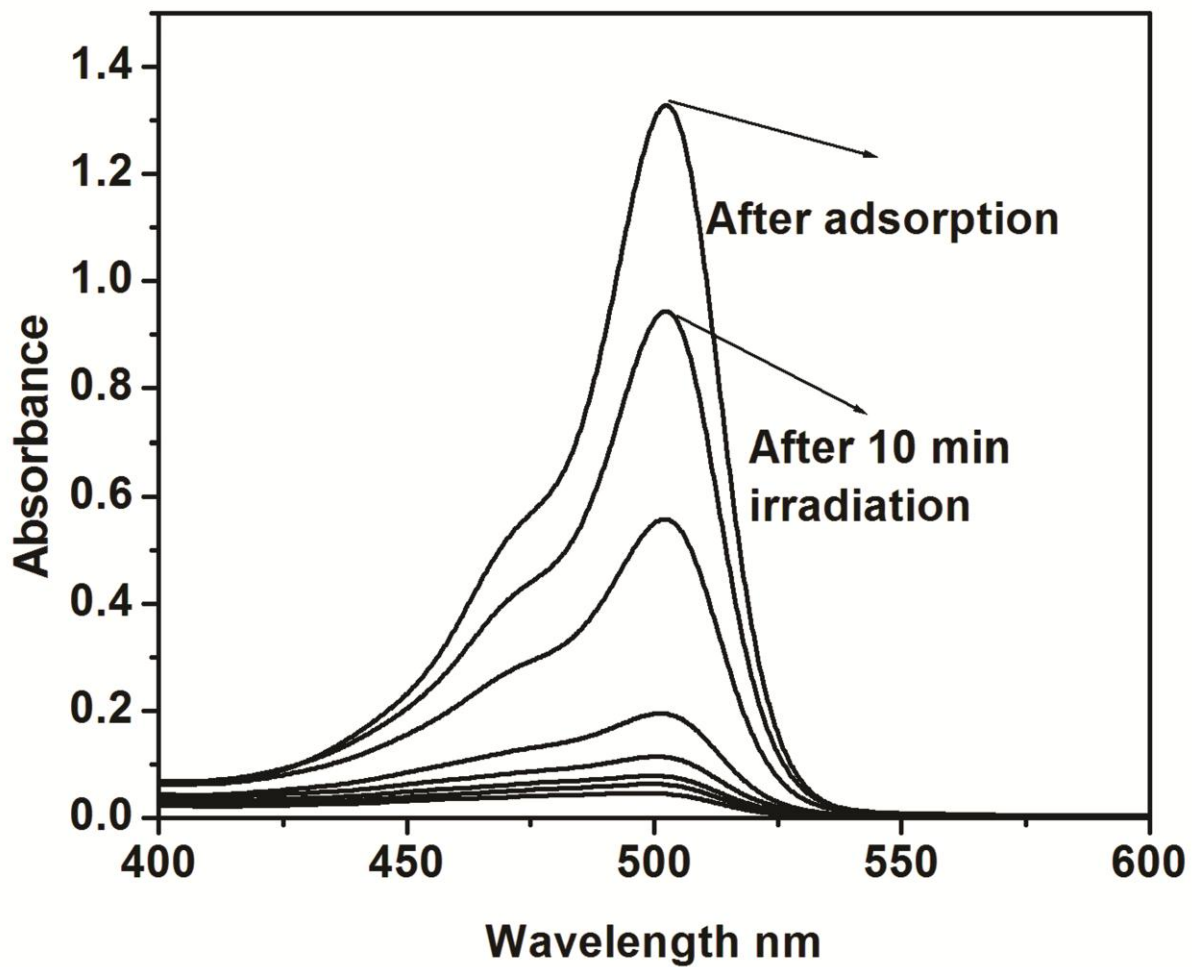
Figure S6. Decomposition of 2, 7-dichloro fluorescein with sulfur doped titania P1.
