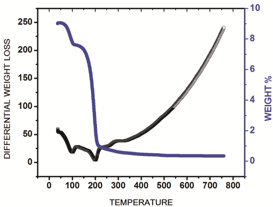
Figure S1. TGA of sulfur doped titania P1.
