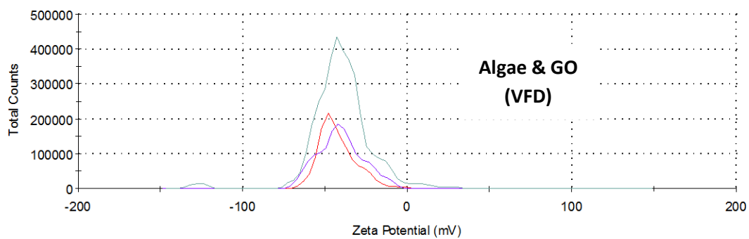
Figure S1. Zeta potential distribution of (a) free cells, (b) GO blank; and GO wrapped cells prepared via (c) sonication, and (d) VFD processing.
