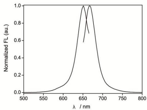
Figure S3. The excitation (left) and emission spectra (right) of 2c
