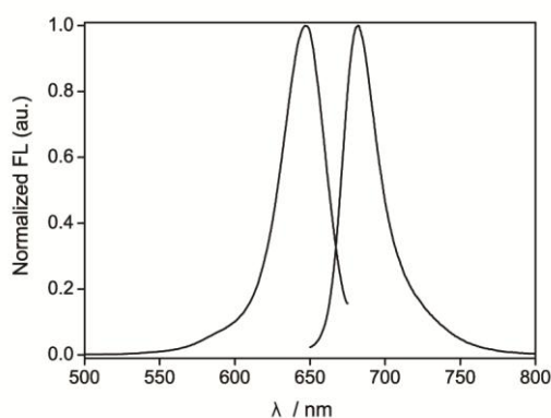
Figure S2. The excitation (left) and emission spectra (right) of 2b
