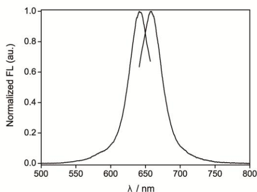
Figure S1. The excitation (left) and emission spectra (right) of 2a
