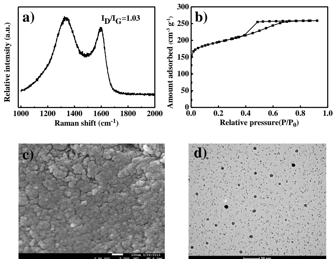
Fig. S1 Raman spectrum (a), N 2 sorption isotherm (b), FE-SEM image (c) and TEM image of activated carbon.
