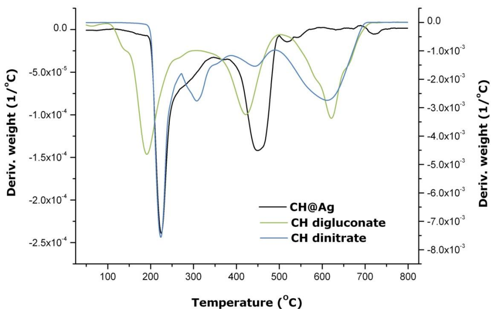
Figure S1: First derivative of the oxidative TGA of CH@Ag (left axis) compared to that of CH dinitrate and that of CH digluconate (right axis)
