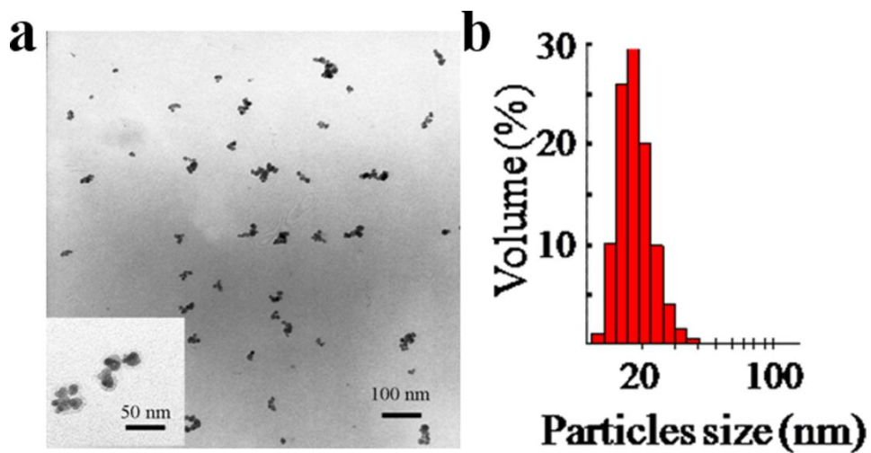
Fig. S1 (a) TEM micrograph and (b) DLS image of Fe 3 O 4 nanoparticles synthesized using a co-precipitation technique.
