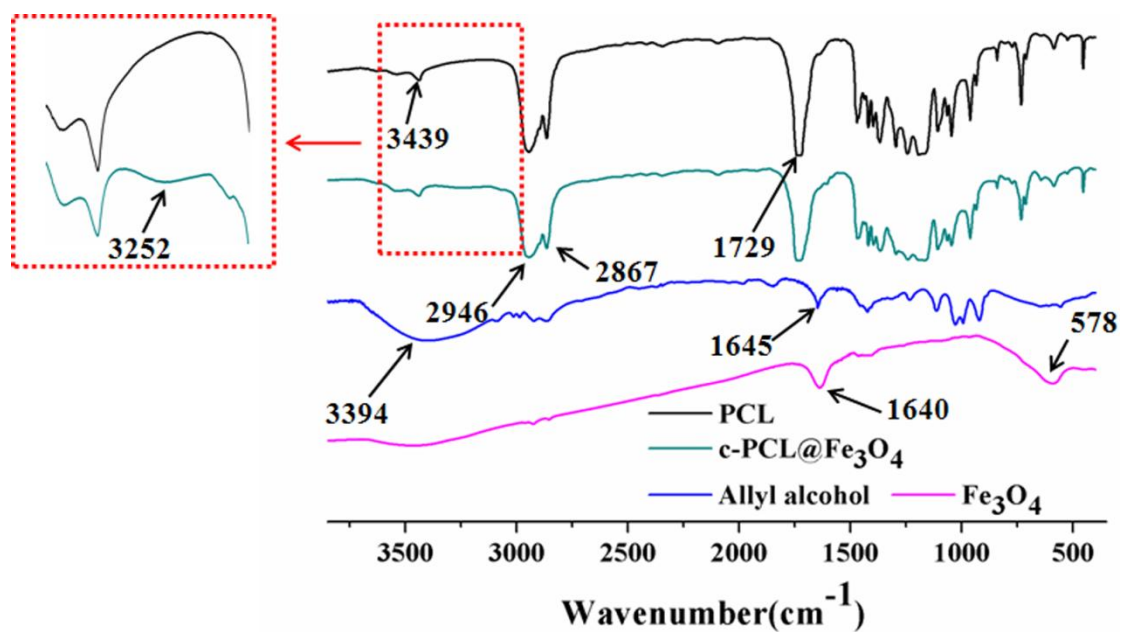
Fig. S2 FT-IR spectra of PCL, Fe 3 O 4 /c- PCL@AL, allyl alcohol and Fe 3 O 4 .
