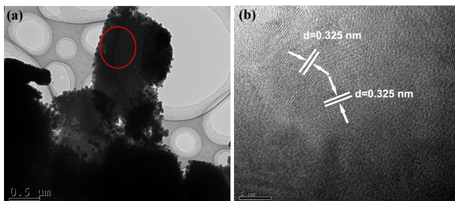
Fig. S1 (a) TEM image of Te plate like crystals, (b) HRTEM image of a single nanoplate taken from the circle of (a).
