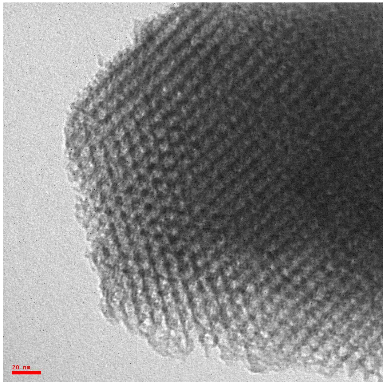
Fig.S 1 TEM image of 1PdNPs/SBA-15 sample
