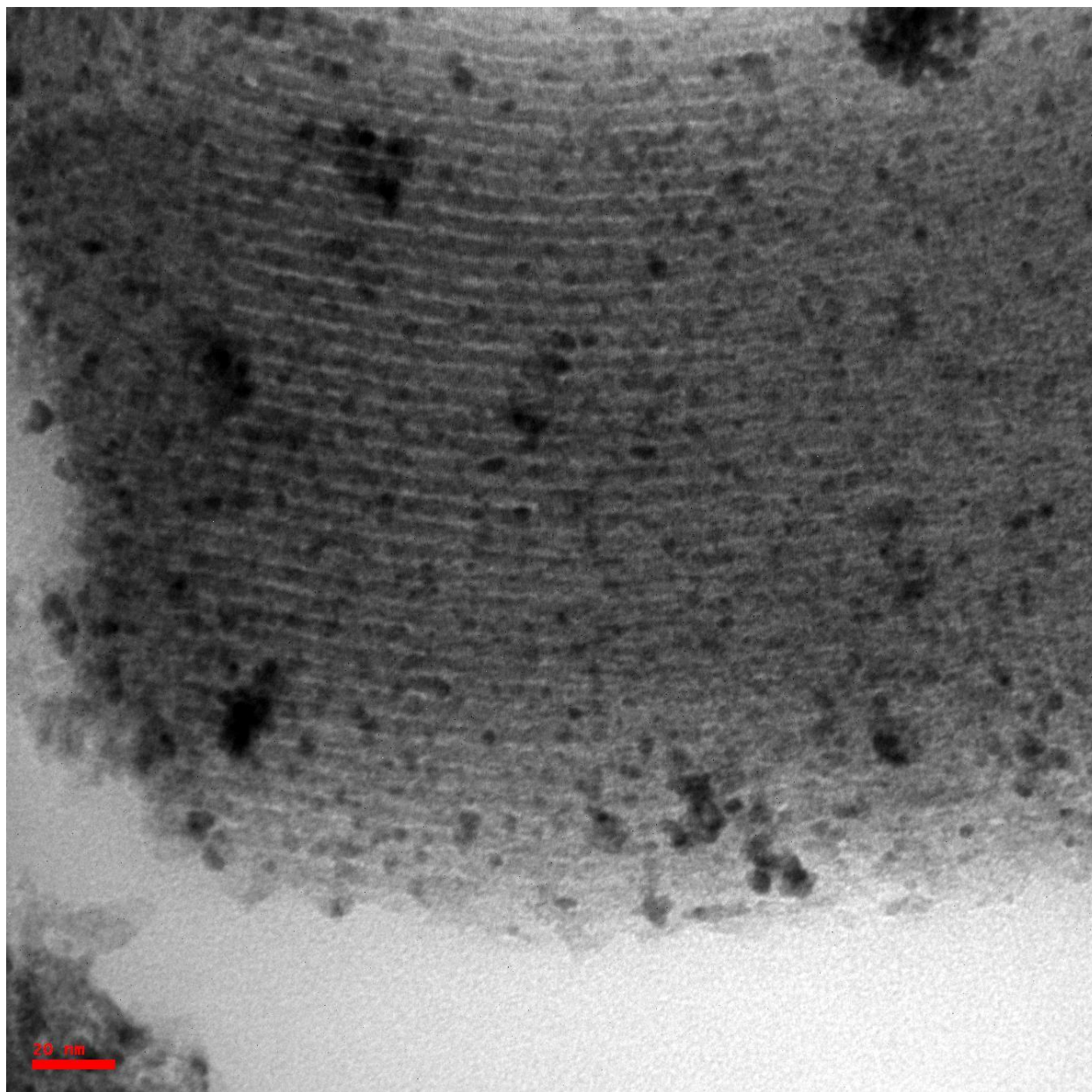
Fig.S 3 TEM image of 7.5PdNPs/SBA-15 sample
