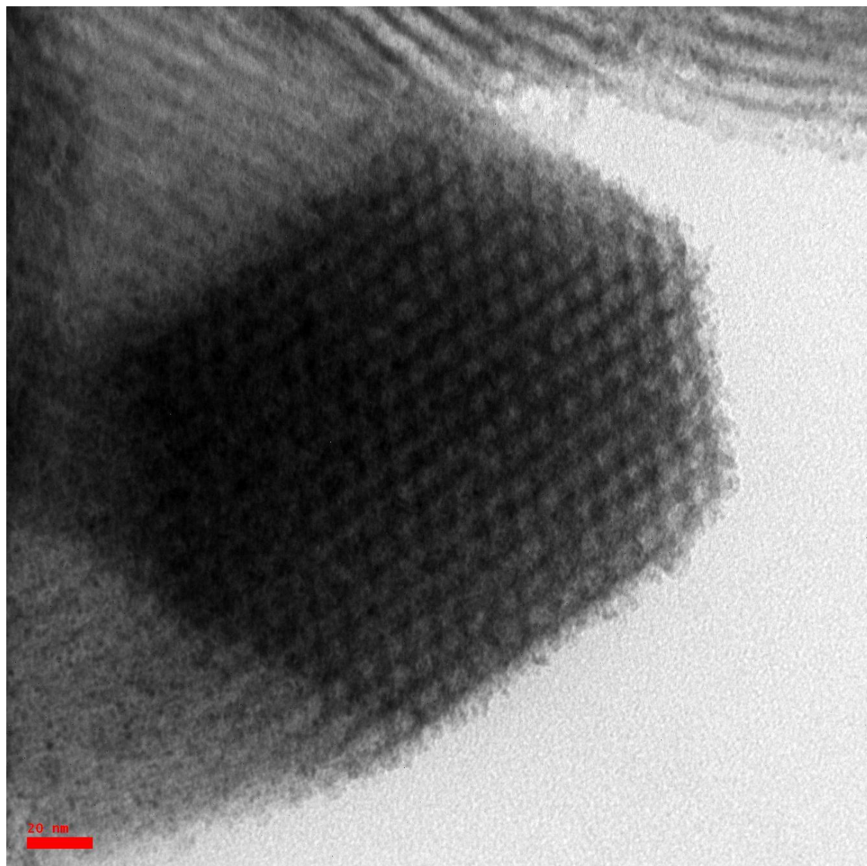
Fig.S 2 TEM image of 2.5PdNPs/SBA-15 sample
