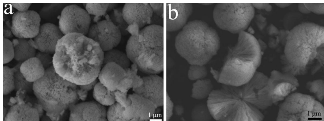
Fig. S2 FESEM images of the samples synthesized at 80 °C using 1.2 mM CTAB at different reaction times: (a) 1 h; (b) 4 h.
