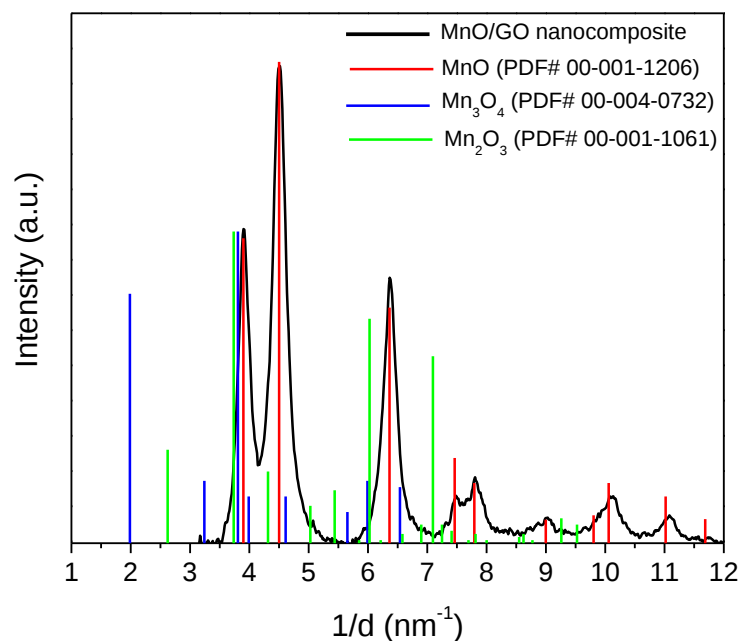
Fig. S1. SAED radial intensity distribution for MnO/GO nanocomposite (black) and ICDD PDF data for MnO (red), Mn 3 O 4 (blue) and Mn 2 O 3 (green).
