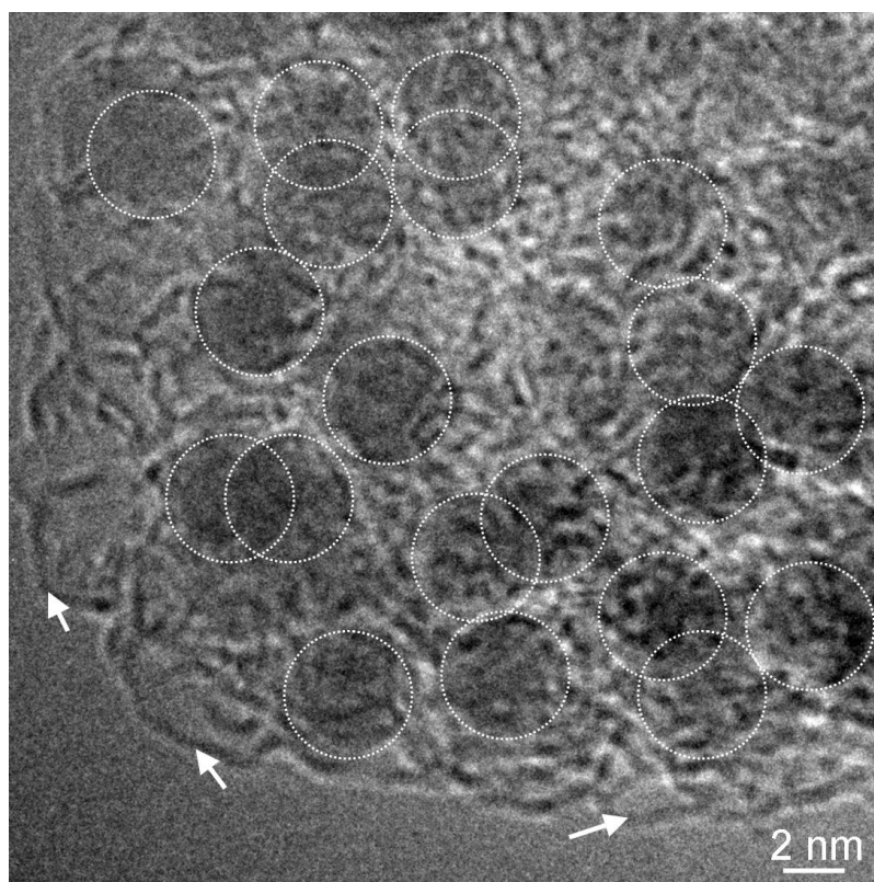
Fig. S2. HRTEM image of MnO/GO nanocomposite. A few GO layers extending to the edge of the flake are marked with arrows. Most of the MnO nanoparticles included in the image are shown with circles.
