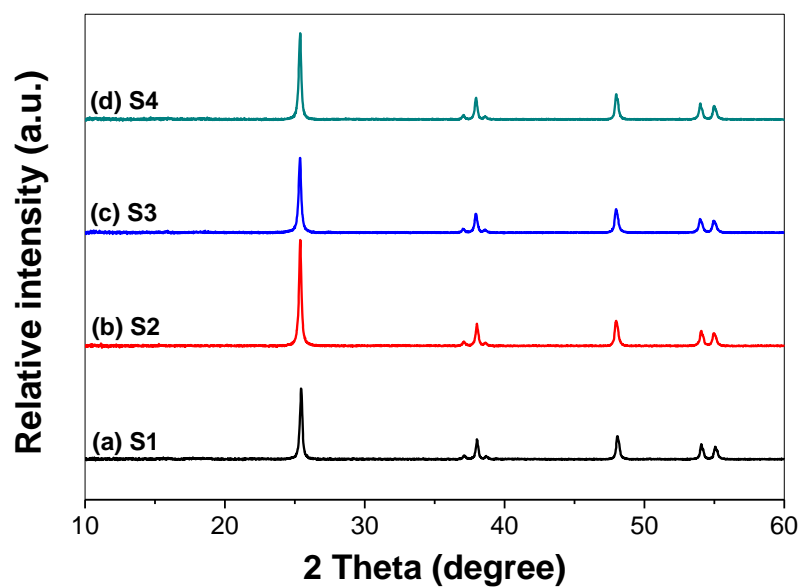
Fig. S1. XRD patterns of TiO 2 samples prepared both in the presence of H 2 O 2 and NH 4 F (see Table 1 for information details).
