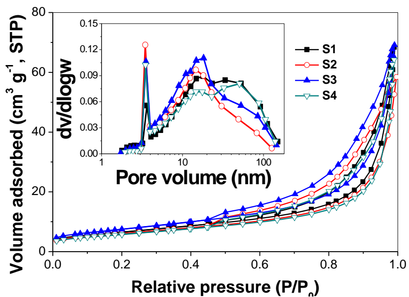
Fig. S2. Nitrogen adsorption–desorption isotherms and the corresponding pore size distributions (inset) of TiO 2 samples prepared both in the presence of H 2 O 2 and NH 4 F (see Table 1 for information details).
