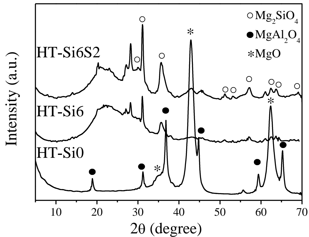
Fig. S2 XRD patterns of various HT samples calcined at 800 .
