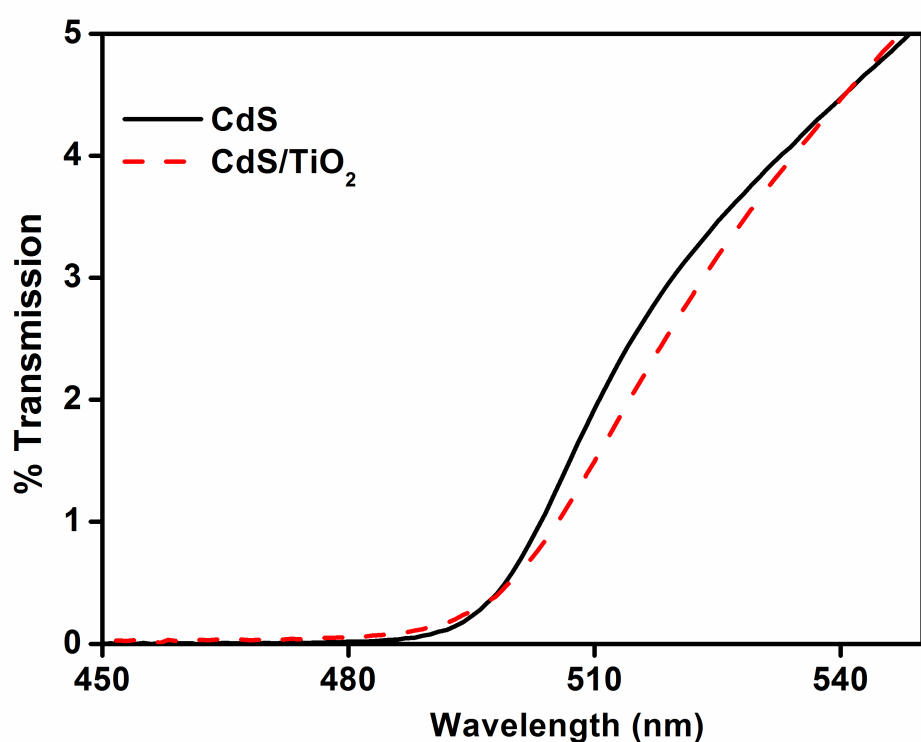
Figure S.I. 2 Transmission Spectra of CdS over FTO and NMP (TiO 2 _CdS) indicating no significant effect on the optical properties of films.
