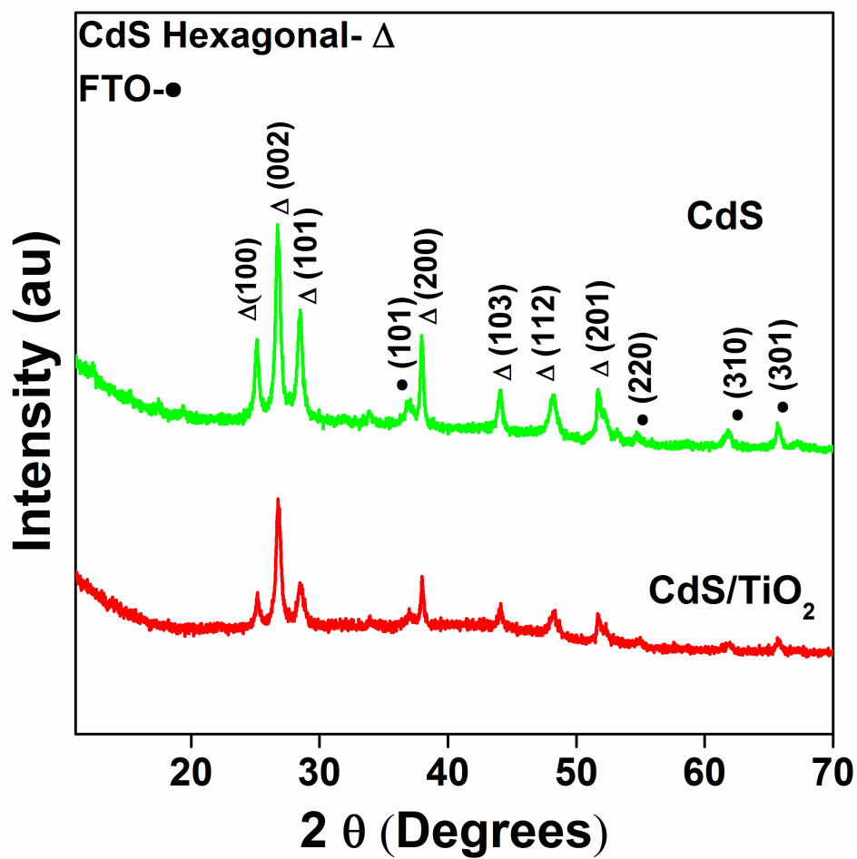
Figure S.I. 1 XRD Spectra of CdS over FTO and NMP (TiO 2 _CdS) indicating the existence of hexagonal CdS phase.
