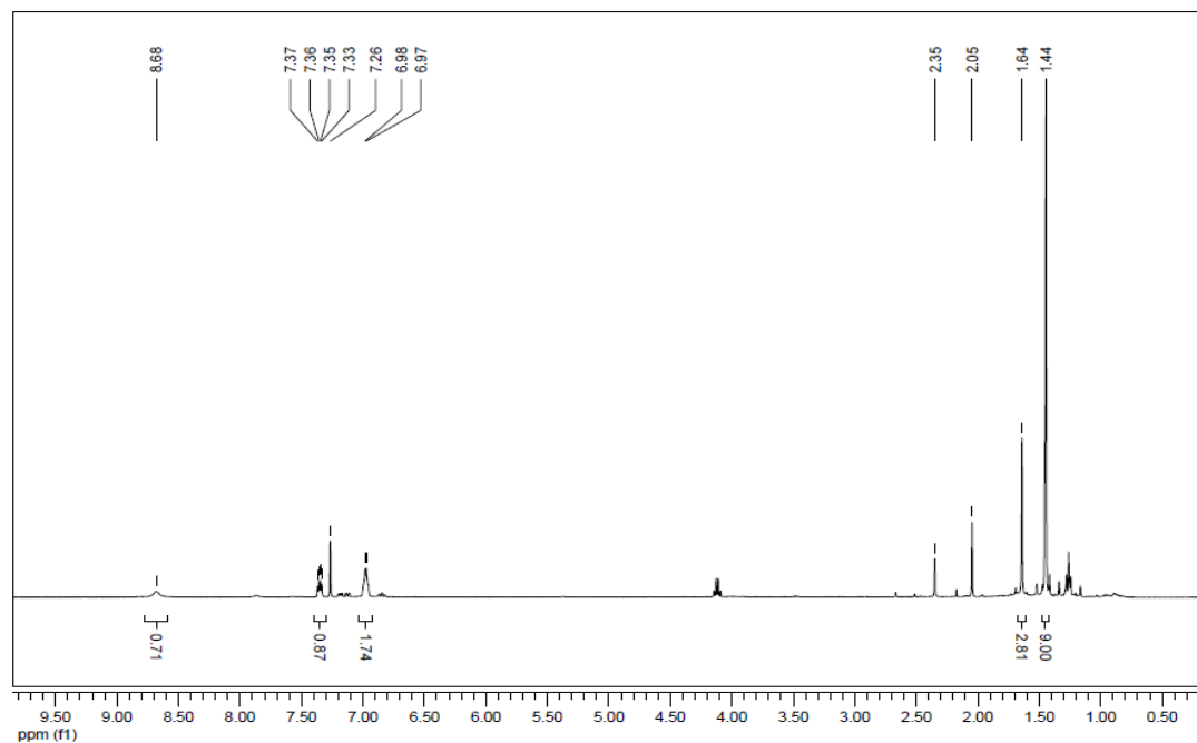
^1\text{H} NMR for 2,3-Diethyl-5-methyl-1H-indole (Table 2, entry 3)
