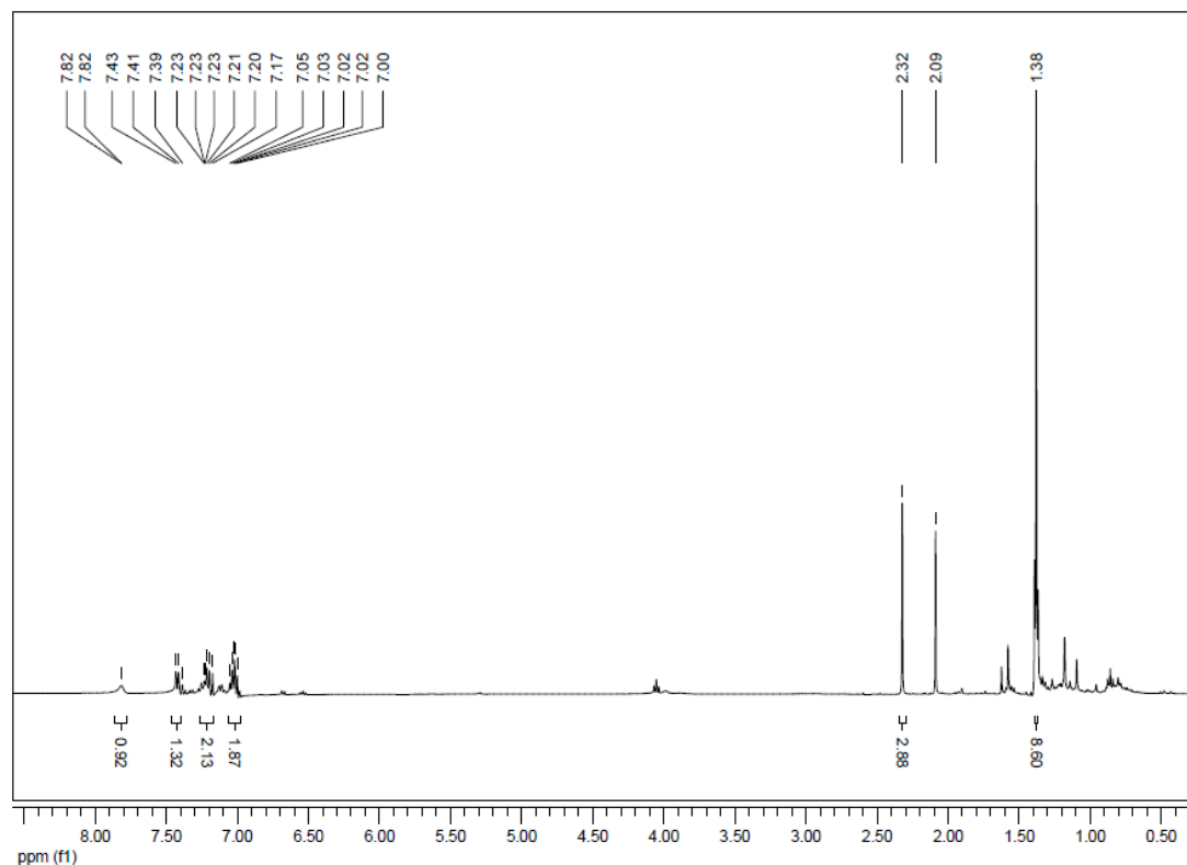
1 H NMR for 3,5-Dimethyl-2-phenyl-1H-indole (Table 3, entry 4, major product)
