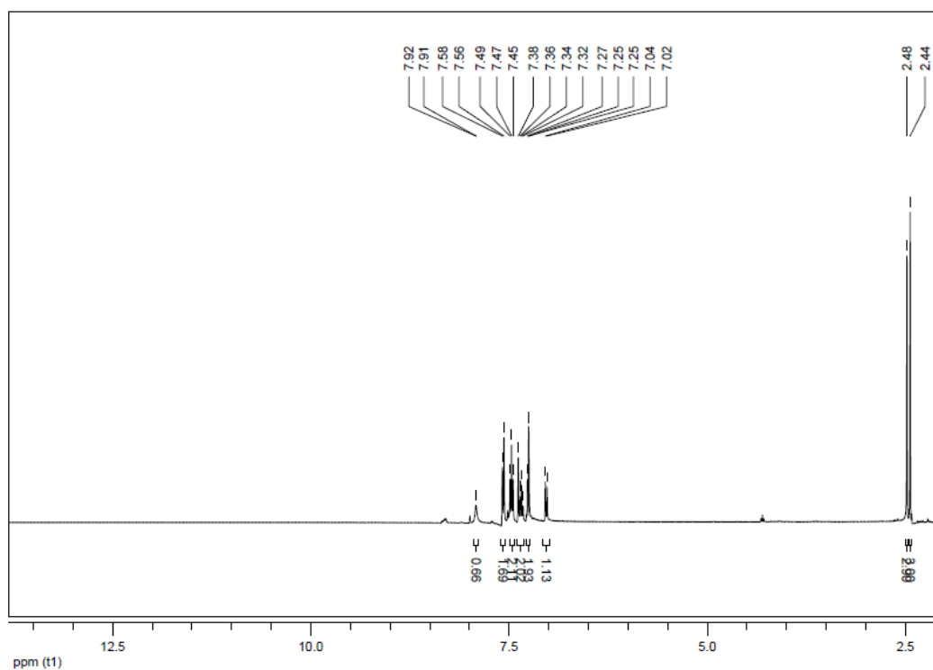
1 H NMR for 3,5-Dimethyl-2-phenyl-1H-indole (Table 3, entry 4, major product)
