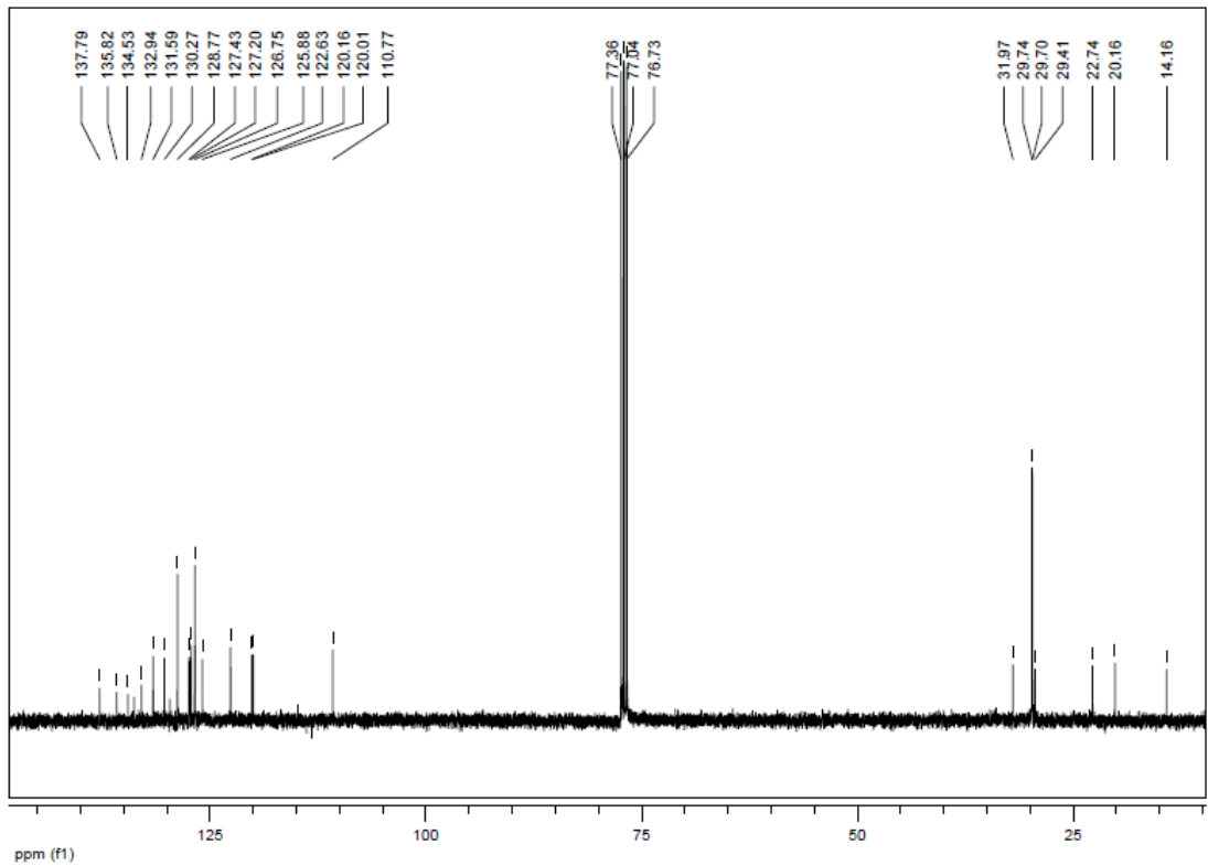
13 C NMR for 3-Phenyl-2-( o -tolyl)-1H-indole (Table 3, entry 12)
