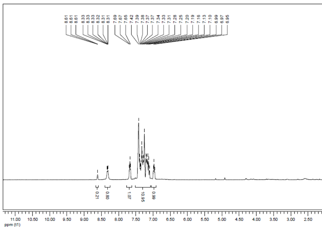
1 H NMR for 2-(3-Fluorophenyl)-3-phenyl-1H-indole (Table 3, entry 11)
