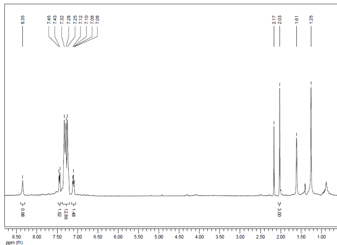
1 H NMR for 3-Phenyl-2-( o -tolyl)-1H-indole (Table 3, entry 12)
