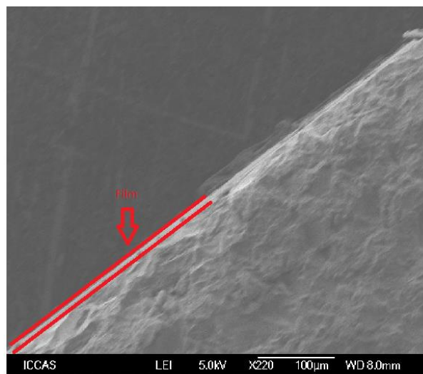
Fig. S1. The cross-section of the Azo-HPC film.
