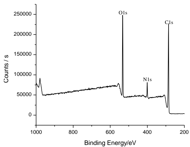
Fig. S3 XPS spectra of the surface of Azo-HPC3 film.
