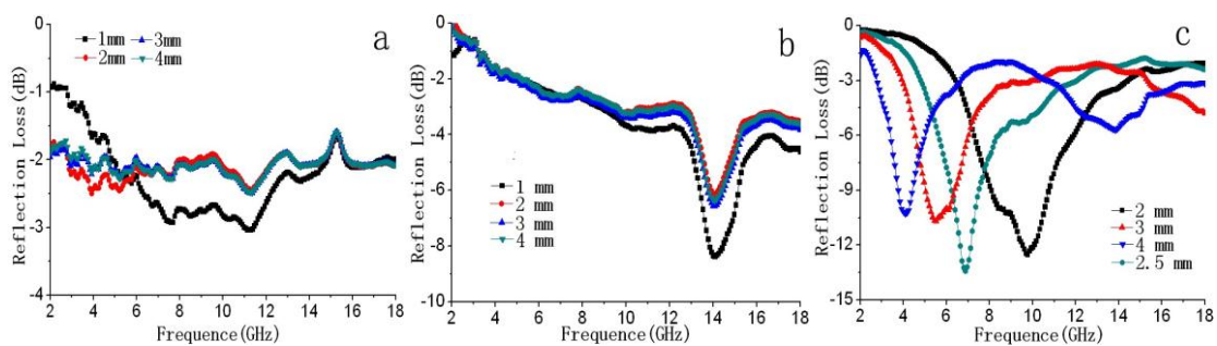
Fig. S3 The R L of RGO-PANI (a), RGO-PPy (b) and RGO-PEDOT (c).
