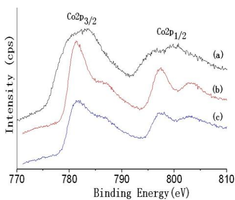
Fig. S2 Co 2p XPS spectra of RGO-PANI-Co 3 O 4 (a), RGO-PPy-Co 3 O 4 (b) and RGO-PEDOT-Co 3 O 4 (c).
