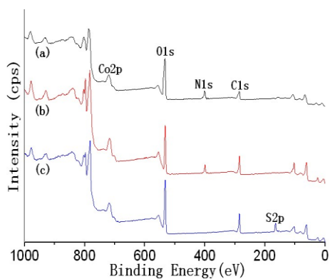
Fig. S1 XPS spectrum of RGO-PANI-Co 3 O 4 (a), RGO-PPy-Co 3 O 4 (b) and RGO-PEDOT-Co 3 O 4 (c).
