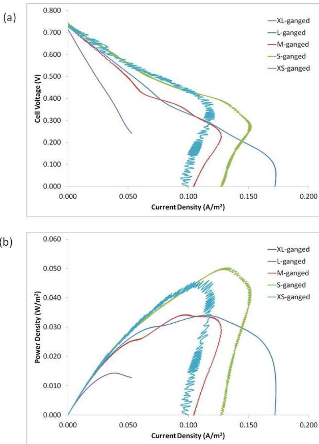
Figure S2. (a) Polarization sweep and (b) power density curves for each of the multi-anode systems. These multi-anode systems were created from steady state anode replicates used in generating data for Figure 2. (XL-ganged = 2 x 6400cm 2 [12,800cm 2 total]; L-ganged = 2 x 1600cm 2 [3200 cm 2 total]; M-ganged = 3 x 400 cm 2 [1200cm 2 total]; S-ganged = 3 x 100 cm 2 [300cm 2 total]; XS-ganged = 3 x 25 cm 2 [75 cm 2 total].
