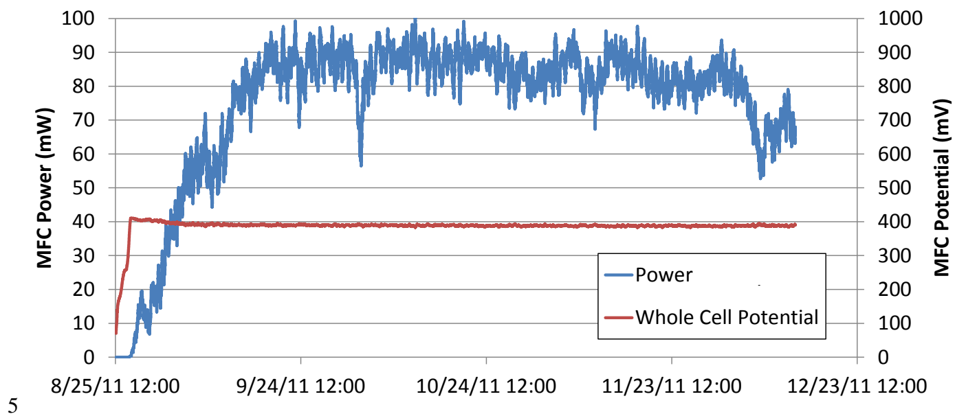
5 Figure S1. Field SMFC power (blue line) and WP (red line) during the deployment period from August to December 2011.
