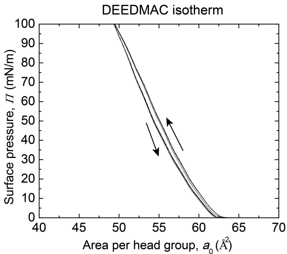
Fig. S1 \Pi - a_0 isotherm of the DEEDMAC monolayer spread at the air-water interface.
