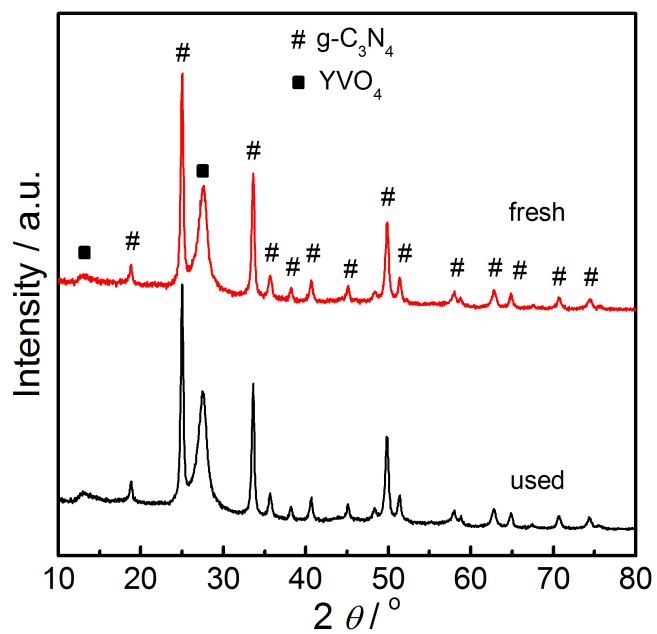
Fig. S4. XRD patterns of 25.8% YVO 4 /g-C 3 N 4 composite before and after reaction.
