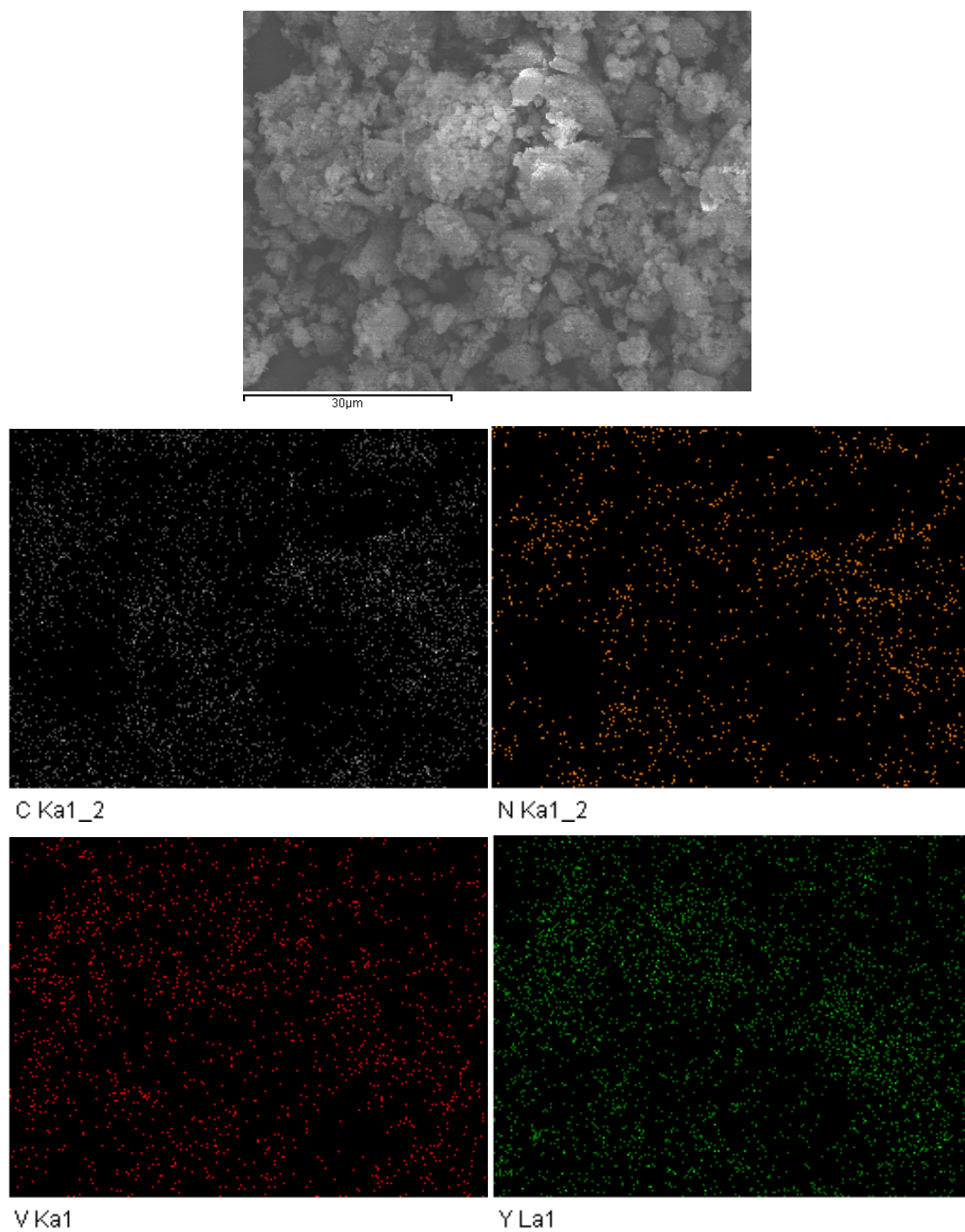
Fig. S3. X-ray elemental maps of 25.8% YVO 4 /g-C 3 N 4 composite.
