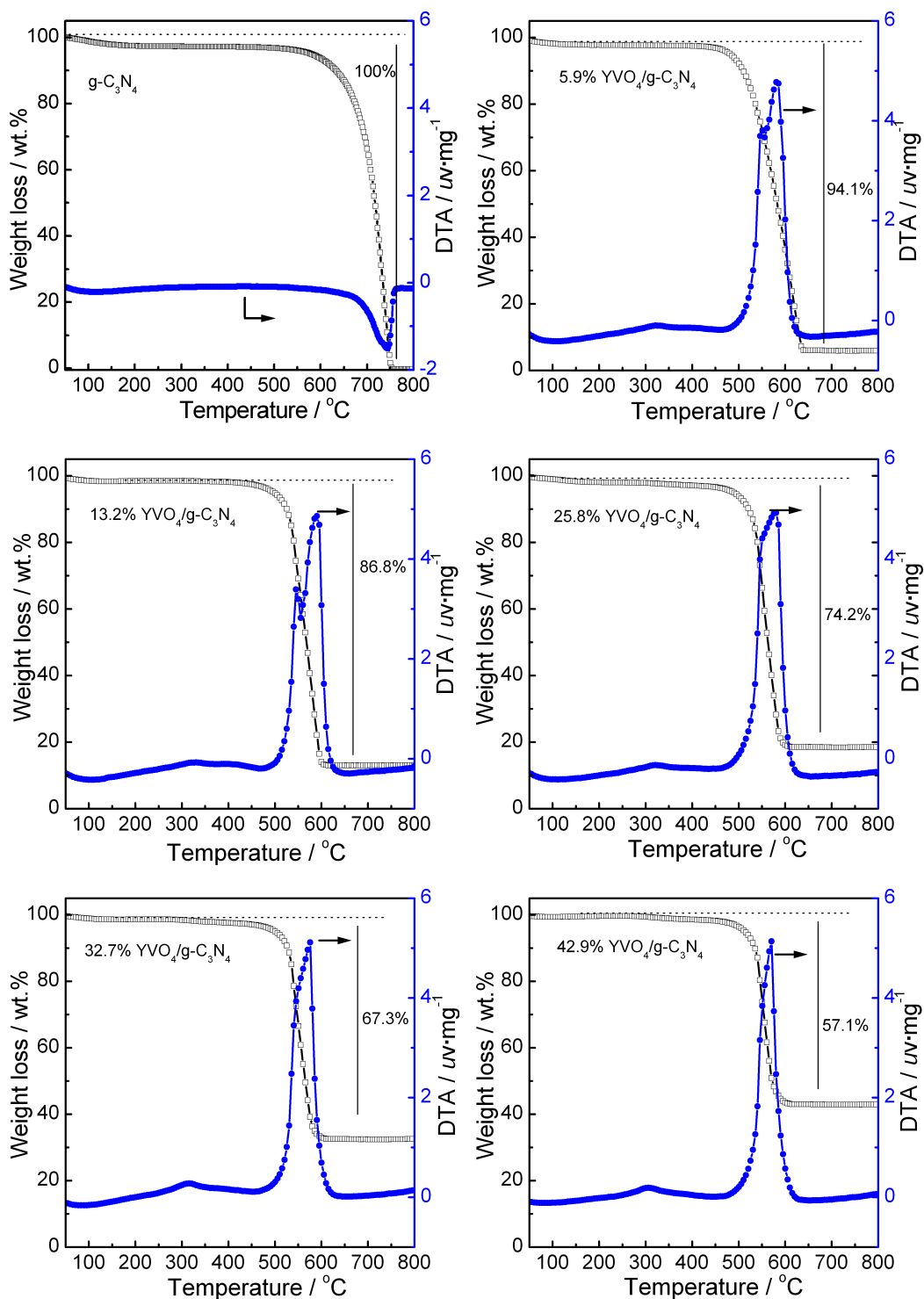
Fig. S1. TG-DTA profiles of \text{g-C}_3\text{N}_4 and \text{YVO}_4/\text{g-C}_3\text{N}_4 composites.
