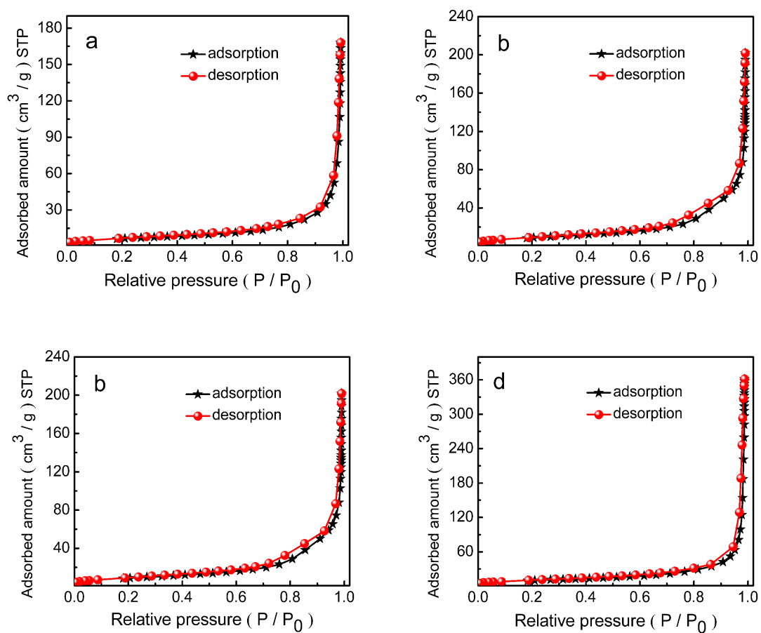
Fig. 1 N 2 adsorption-desorption curves of (a) S2, (b) S3, (c) S5, and (d) S6.
