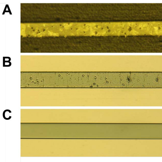
ESI Figure 1. Channel roughness resulting from photoplot masks. (A) Photograph of a 100- \mu\text{m} -wide channel on the photoplot itself. (B) SU-8 channel produced from the section of photoplot shown in (A). (C) 100- \mu\text{m} -wide SU-8 channel created using a glass photomask. Channel heights are 25 \mu\text{m} .
