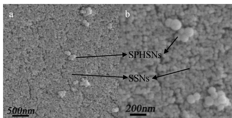
Figure S2. SEM images of (SSNs) 1 /(SPHSNs) 1 coating on Fresnel lens. (b) is the magnified image of (a).
