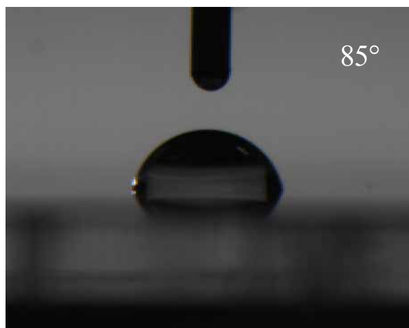
Figure S1. WCA on the smooth surface of Fresnel lens prior to any surface modification.
