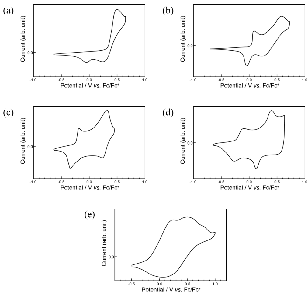
Fig. 1S. Cyclic voltammograms of E n Ts in dichloromethane solution. (a) E 3 T , (b) E 6 T , (c) E 7 T , (d) E 9 T and (e) E 11 T . Scan rate: 50 mV s -1 . Electrolyte: Bu 4 NClO 4 (0.1 M).
