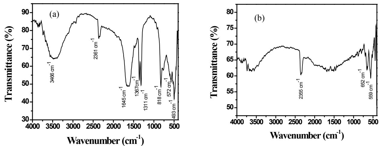
Figure S2. FTIR spectrum of (a) oxalate precursor (b) \text{NiCo}_2\text{O}_4 nanostructures (NCO-2)
