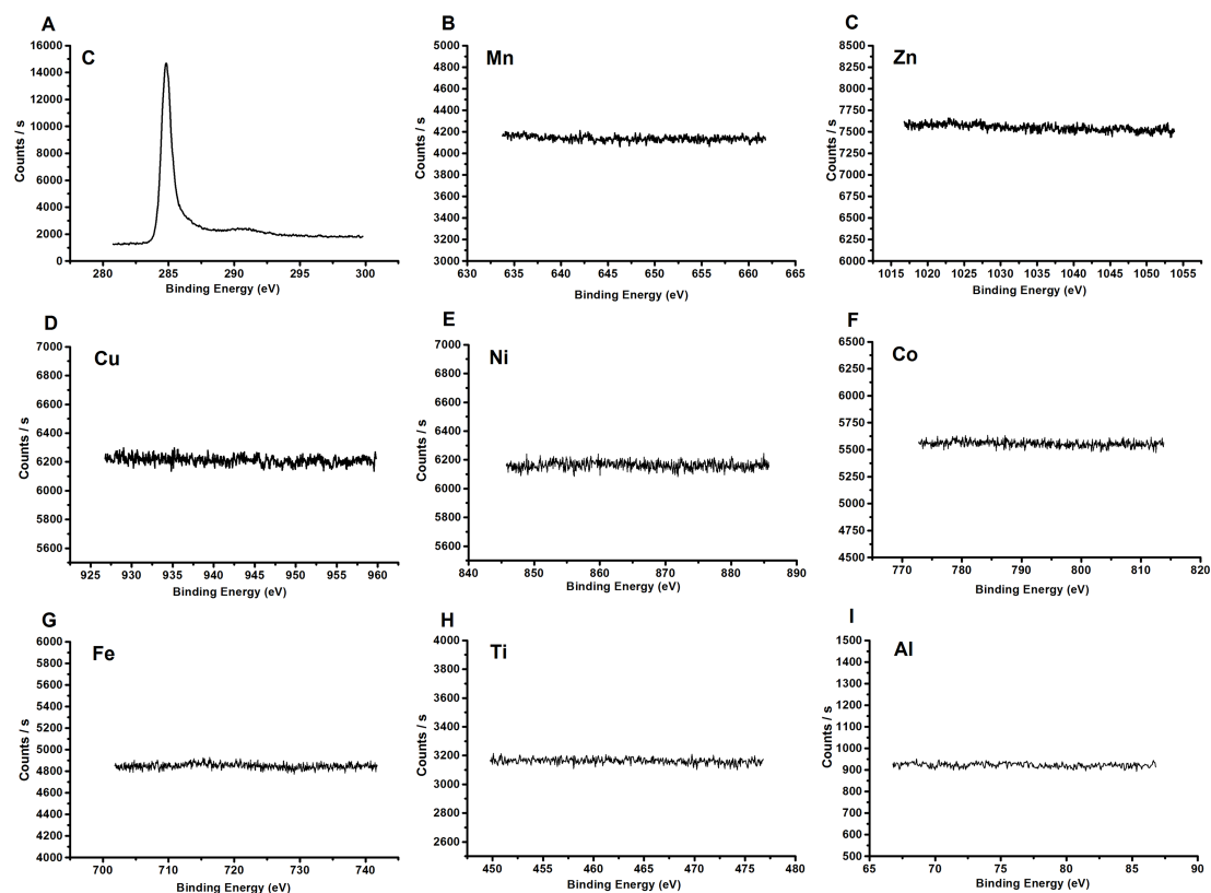
Figure S1. XPS spectra of SWCNTs. A: C 1s, B: Mn 2p, C: Zn 2p, D: Cu 2p, E: Ni 2p, F: Co 2p, G: Fe 2p, H: Ti 2p, I: Al 2p.
