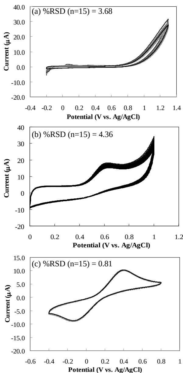
Fig. S1 CV responses of SPGE towards (a) 5 mM \text{H}_2\text{O}_2 , (b) 5 mM NADH and (c) 1 mM \text{K}_4\text{Fe}(\text{CN})_6 solutions for 15 consecutive cycles. Scan rate was 100 \text{ mVs}^{-1} .
