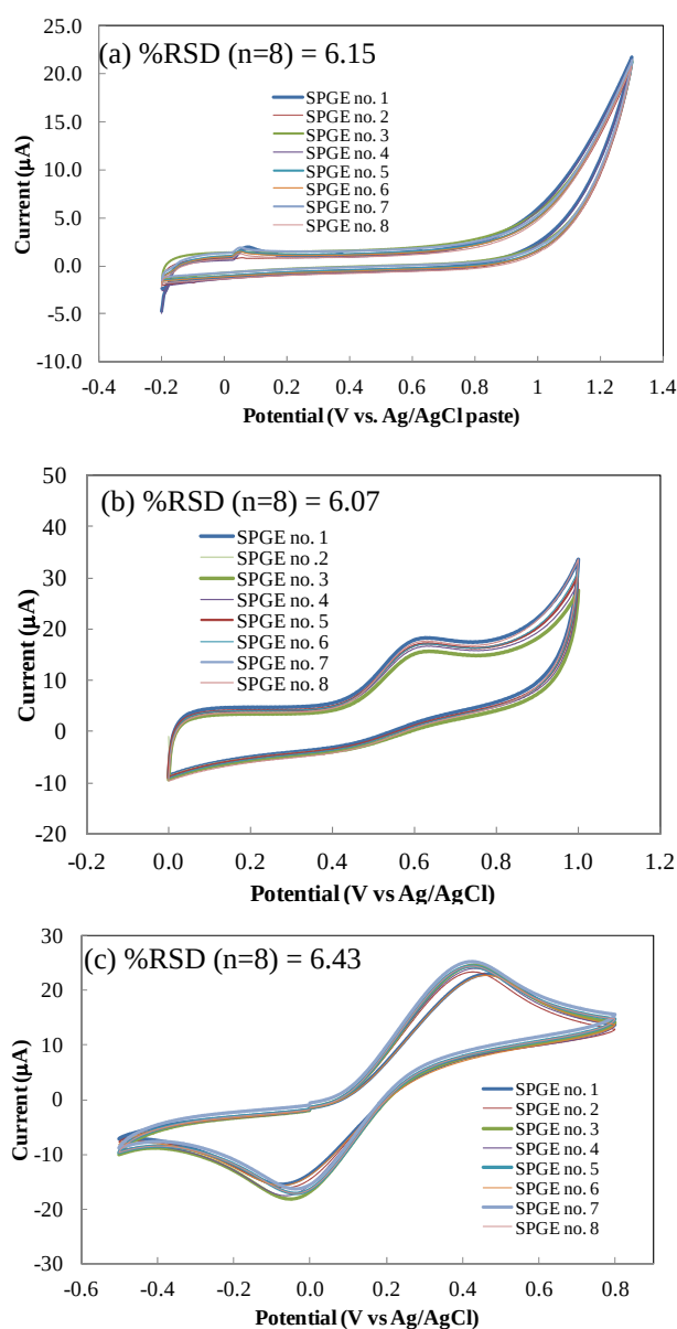
Fig. S2 CV responses of 8 SPGEs fabricated in the same batch towards (a) 5 mM \text{H}_2\text{O}_2 , (b) 5 mM NADH and (c) 1 mM \text{K}_4\text{Fe}(\text{CN})_6 solutions. Scan rate was 100 \text{ mVs}^{-1} .
