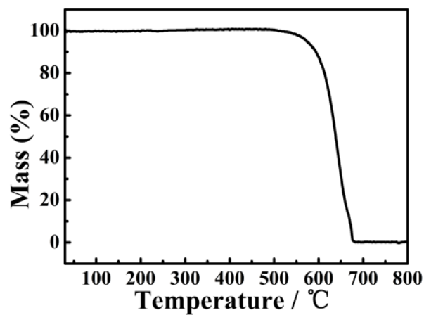
Figure S-1. TGA curve of PCS-120.
