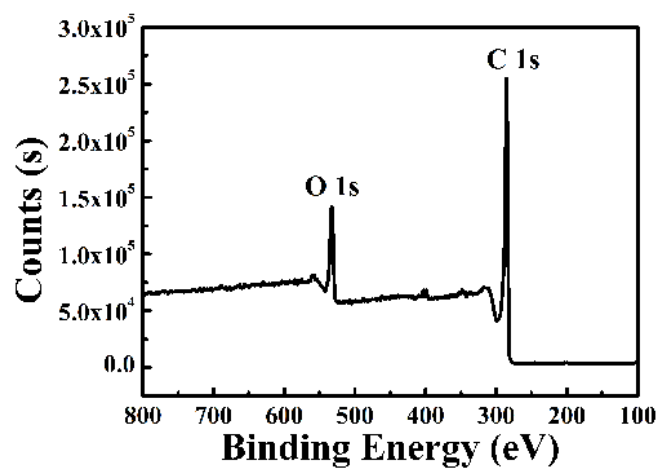
Figure S-2. XPS scan of PCS-120.
