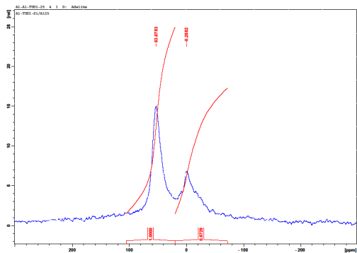
Figure S1 ^{27}\text{Al} MAS NMR spectra of the Al-TUD-1 25 material
