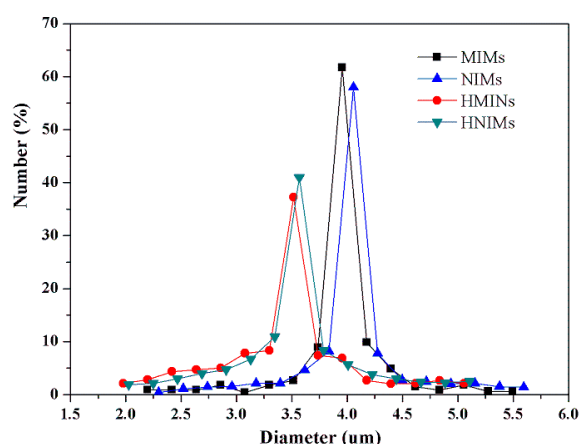
Fig. S1. Diameter distributions calculated from dynamic light scattering measurements for MIMs HMIMs, NIMs and HNIMs.
