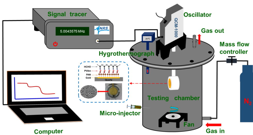
Fig. S2 Schematic diagram of a gas testing system for formaldehyde monitoring.
