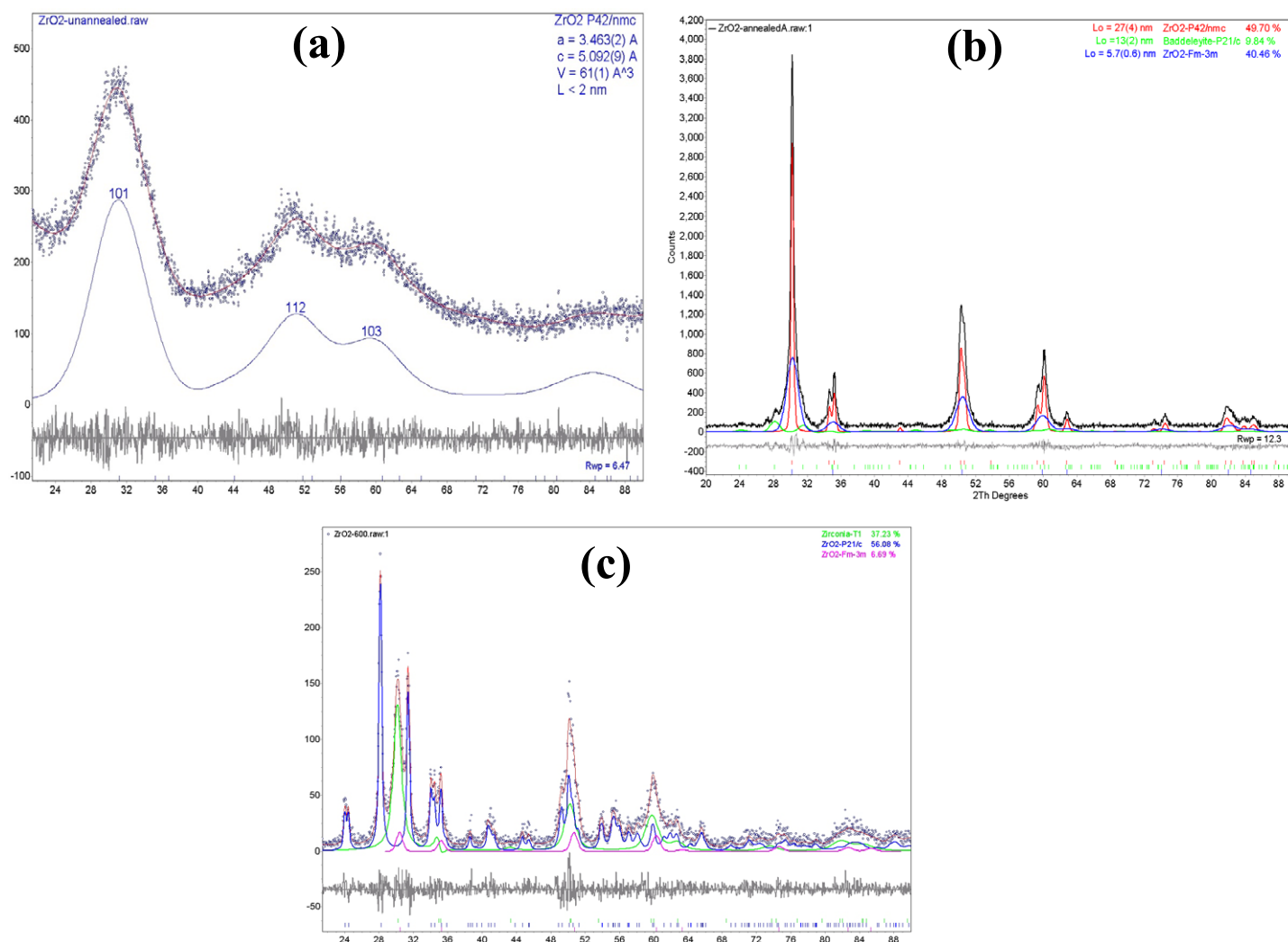
Observed and calculated diffraction pattern using Rietveld refinement for ZrO 2 nanoparticles a) before annealing b) annealed at 400 °C c) annealed at 600 °C
