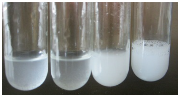
Figure S1 Reaction mixture of the Mannich reaction with different catalysts at the beginning.
