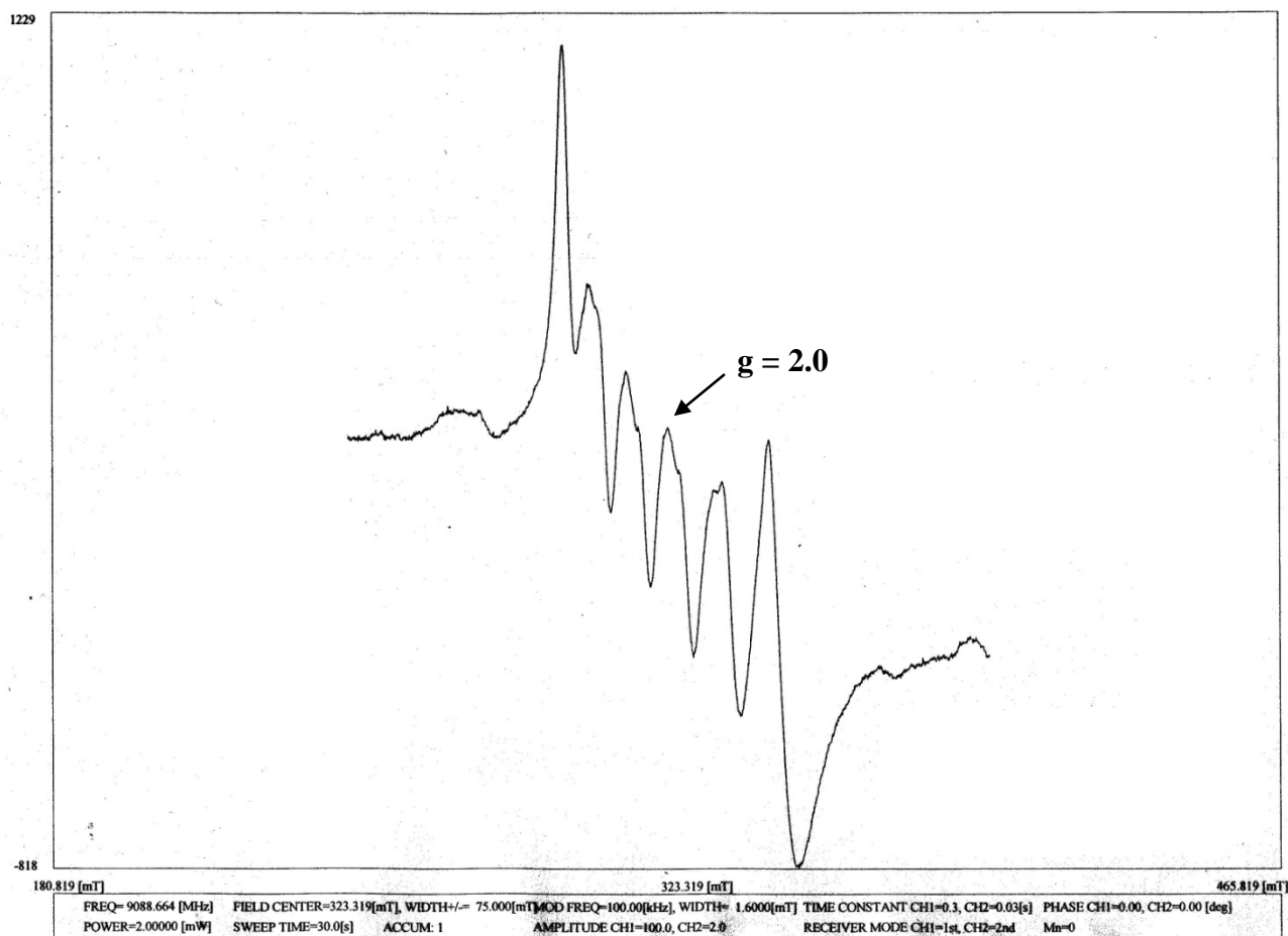
Fig. S1 X-band EPR spectra of [Mn(L)]1- 4 at LNT. Instrumental parameters: microwaves, 9.08 GHz at 2 mW; modulation 100 KHz.
