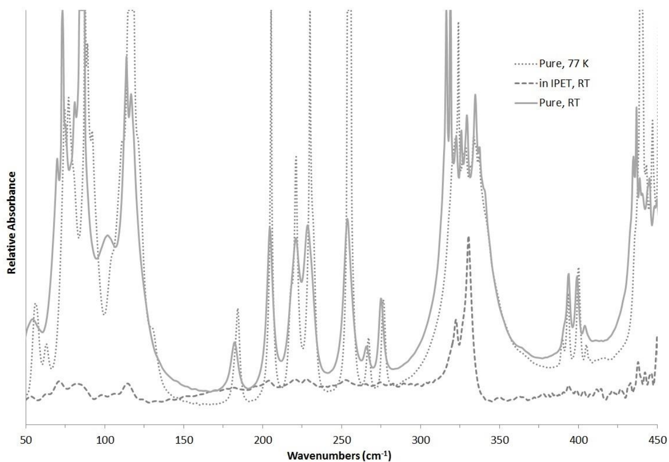
Figure S1: Absorption spectra of \text{AuPPh}_3\text{Cl} pure disks at room temperature and 77 K, as well as diluted in polyethylene at room temperature.
