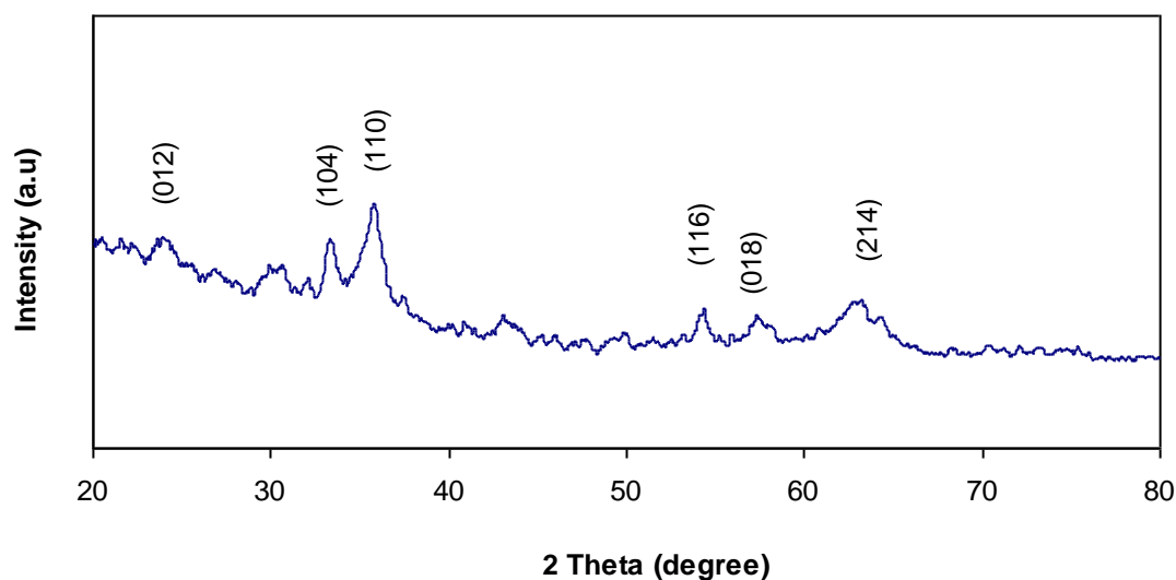
Figure S2. XRD pattern of Fe 2 O 3 /C annealed at 300 °C
