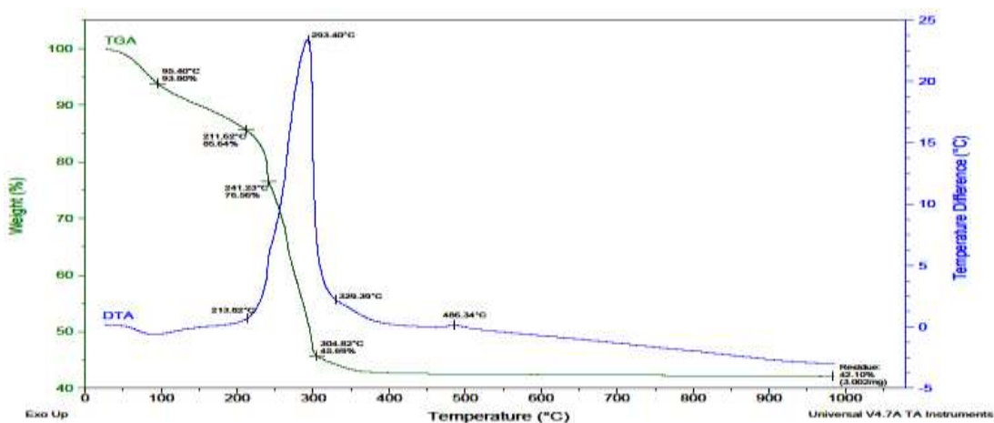
Figure S1. TG – DTA traces illustrating the thermal decomposition of the as prepared material.
