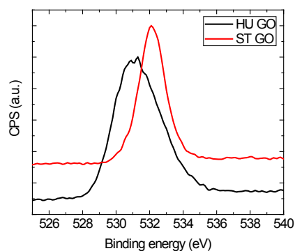
Figure S3. Detail of high resolution XPS spectra of graphite oxides O 1s peak for ST-GO and HU-GO samples used for fluorinations.
