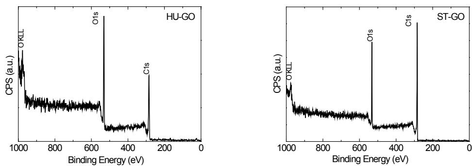
Figure S1. Wide-range XPS spectra of graphite oxides ST-GO and HU-GO.
