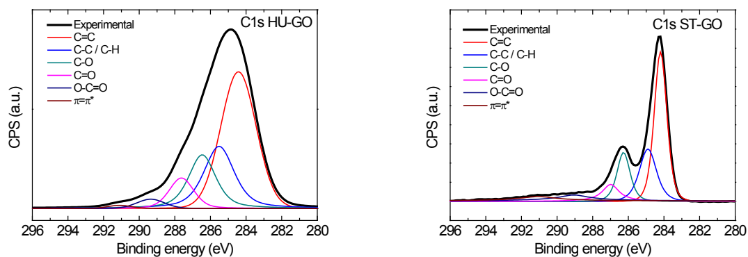
Figure S2. Detail of high resolution XPS spectra of graphite oxides C 1s peak for ST-GO and HU-GO samples used for fluorinations.
