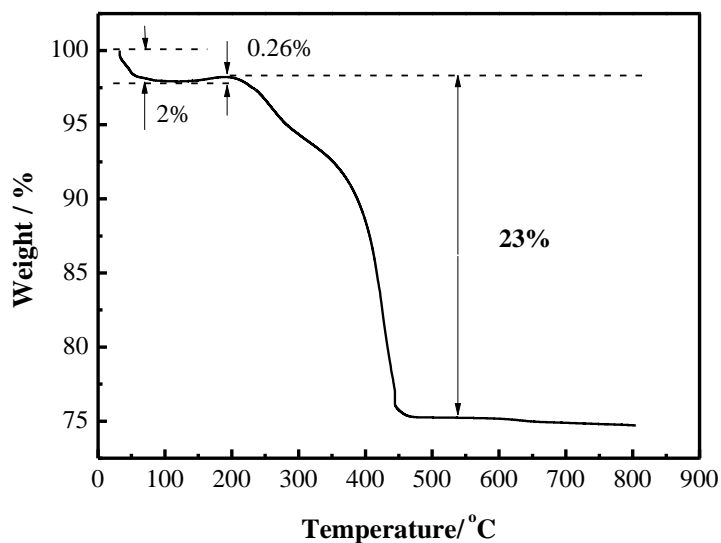
Fig. S1 TG plot of the H-Fe 3 O 4 -MS/GNS composite.
