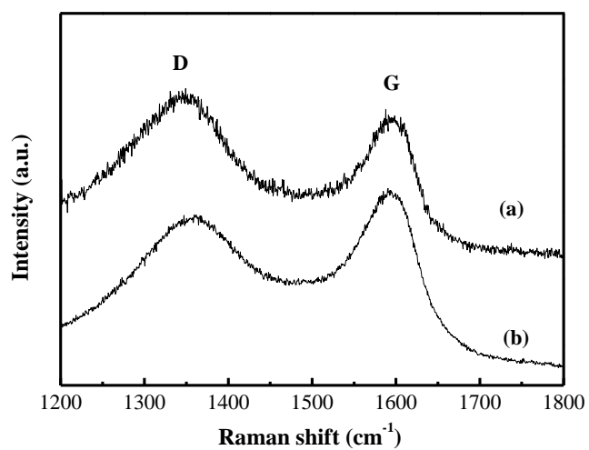
Fig. S2 Raman spectra of (a) H-Fe 3 O 4 -MS/GNS composite, and (b) GO.
