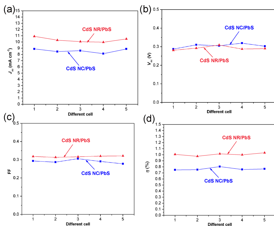
Fig. S1 Photocurrent density–voltage ( J – V ) parameters of five CdS NR/PbS 3D heterojunction solar cells and five CdS NC/PbS planar heterojunction solar cells.
